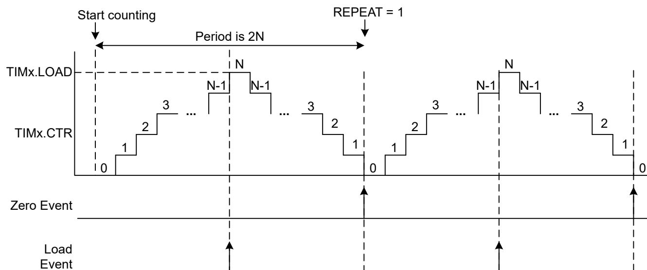
Figure 17-8. Up-down Counting Mode and Event Generation, CVAE = 2
