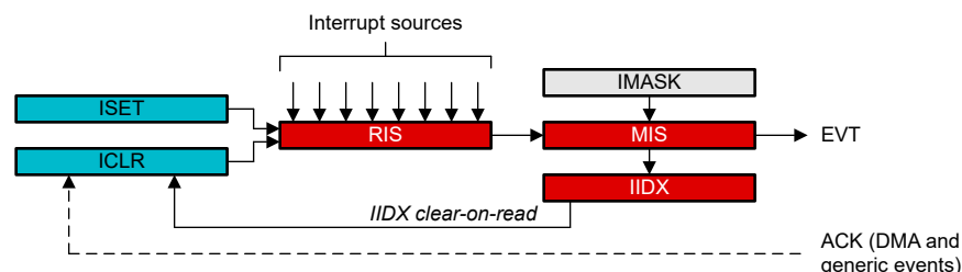
Figure 7-6. Event Management Register Relationship
