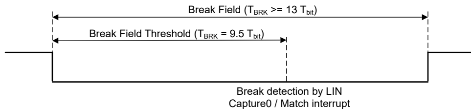
Figure 12-6. LIN Break Field Detection
