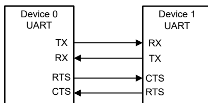
Figure 12-9. Flow Control
