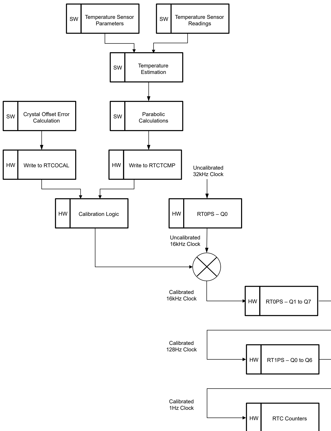
Figure 19-2. RTC Calibration
