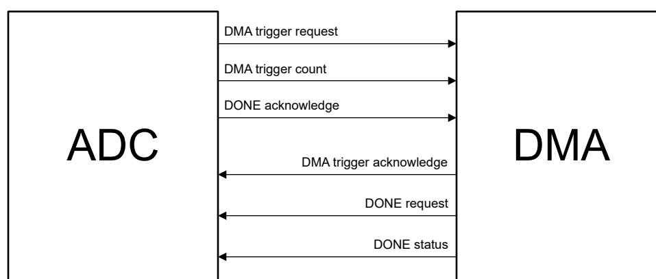
Figure 10-4. Internal ADC-DMA Interface
