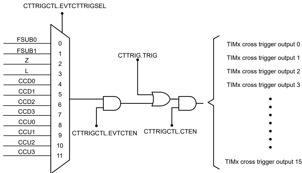
Figure 17-39. Main Timer Cross Trigger Output Configuration
