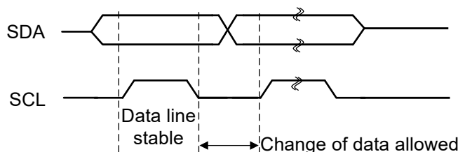
Figure 14-4. Data Change Period
