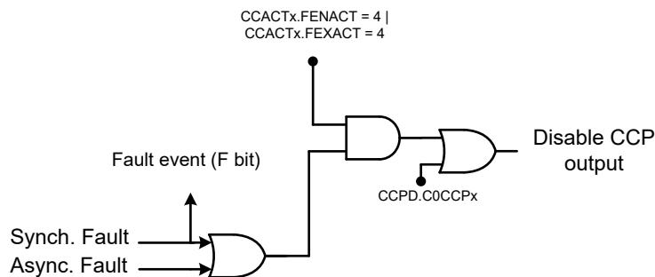
Figure 17-36. Fault Output Generation Connections
