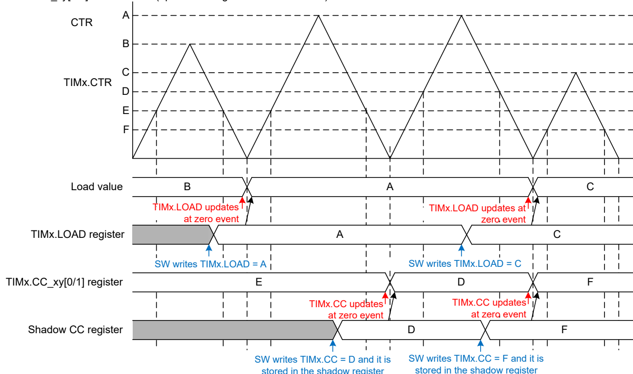
Figure 17-25. Shadow Load and Shadow Compare Taking Effect at Zero Event in Up/Down Mode
