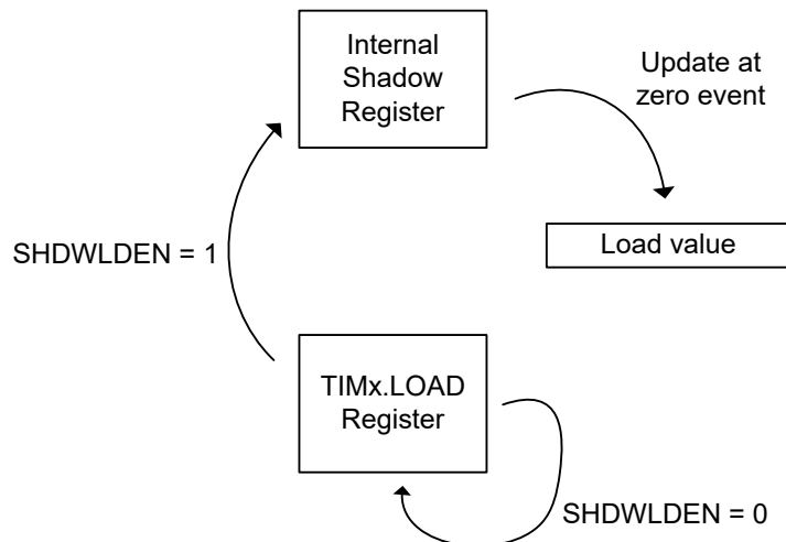
Figure 17-24. Load value updates for TIMx instances when EN=1
