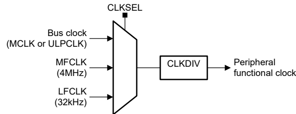
Figure 2-7. Peripheral Clock Selection Mux and Divider
