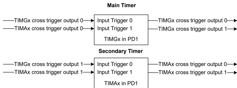
Figure 17-38. Cross Trigger Connections for Main Timer (TIMGx) and Secondary Timer (TIMAx) in Power Domain 1
