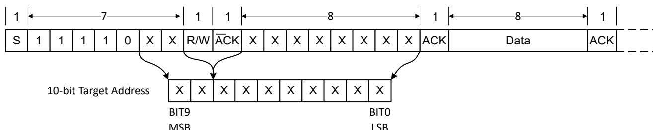
Figure 14-7. Data Format with 10-Bit Address
