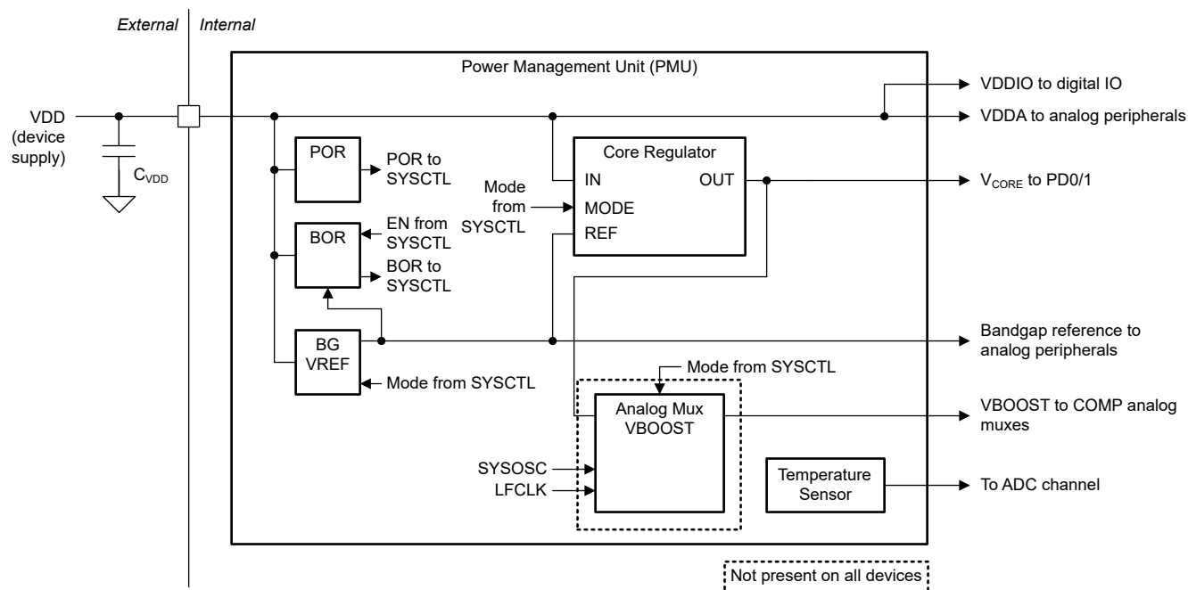
Figure 2-3. MSPM0Hxx PMU Block Diagram
