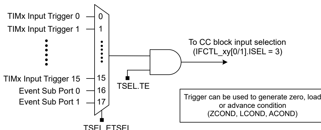
Figure 17-40. Secondary Timer Cross Trigger Input Configuration
