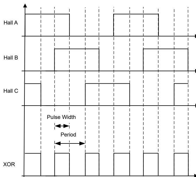
Figure 17-22. Hall 3-Input XOR Signal used with Pulse Width or Period Capture for Speed Computation
