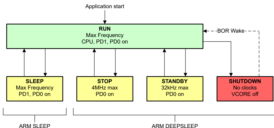
Figure 2-2. MSPM0Hxx Operating Modes
