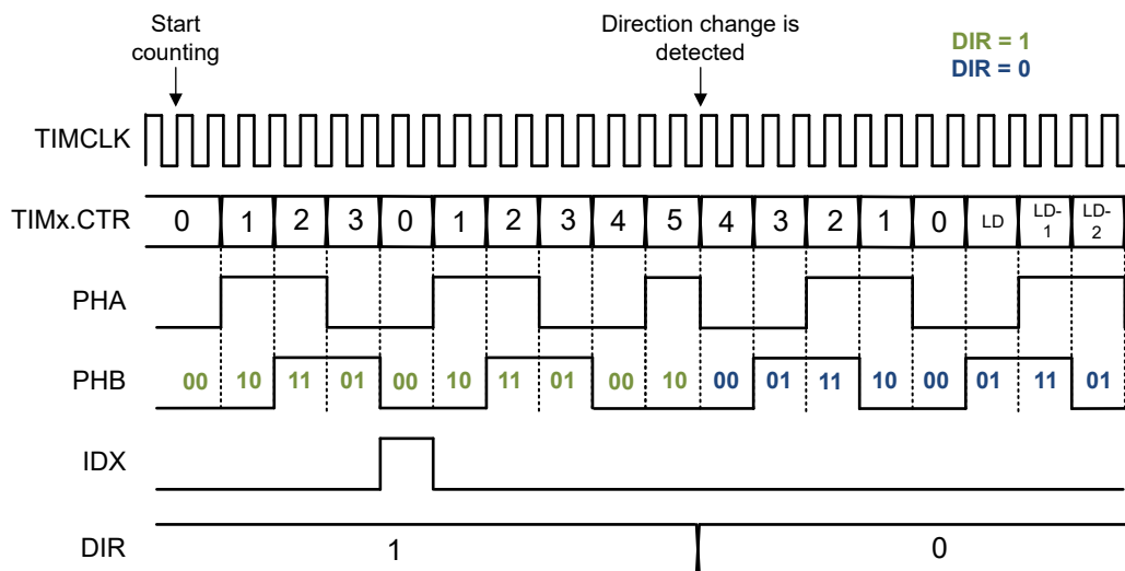
Figure 17-20. 2-Signal QEI with Index Input Operation
