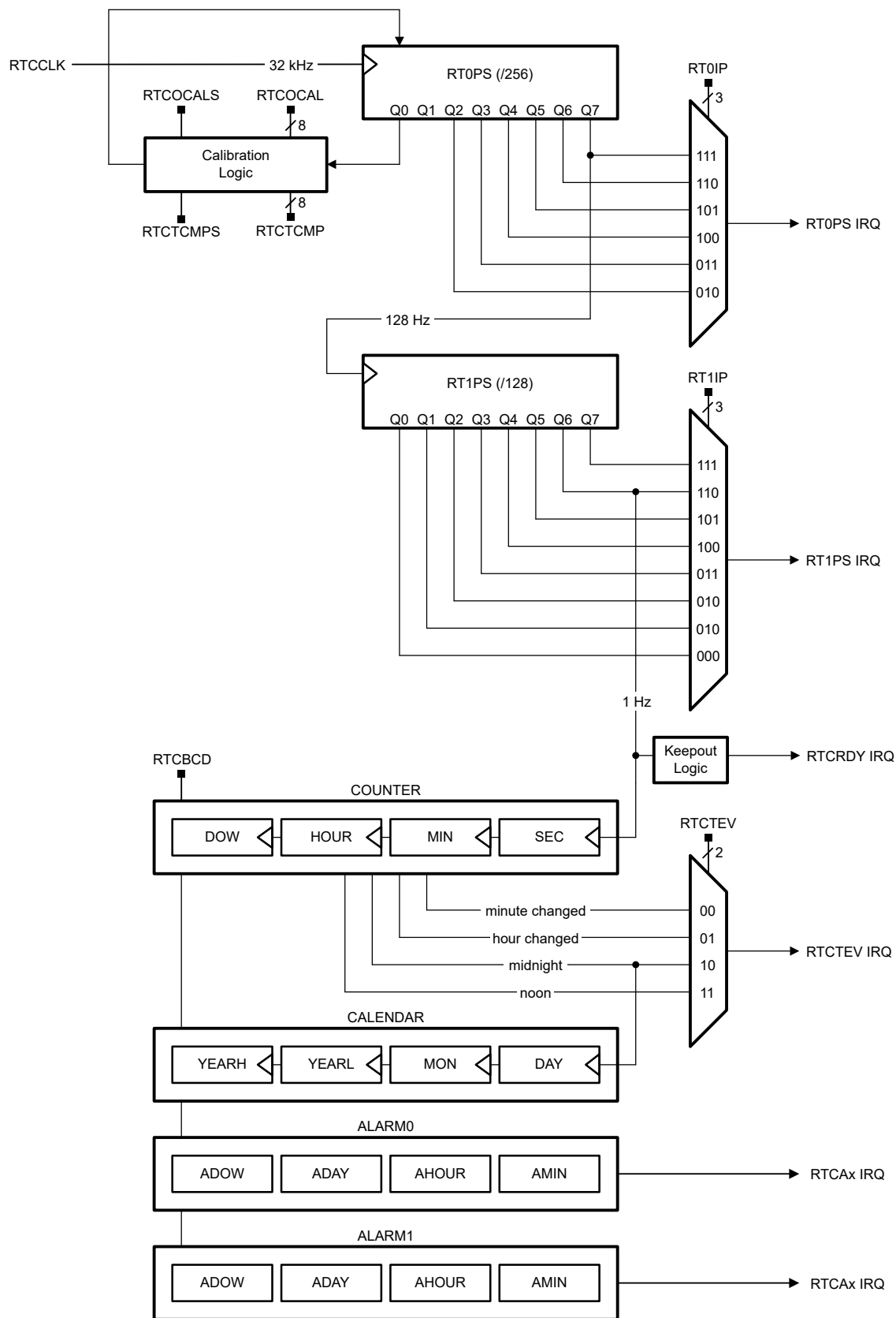
Figure 19-1. RTC Block Diagram
