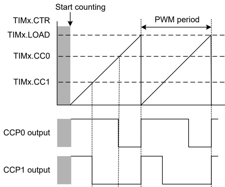
Figure 17-29. Edge-Aligned PWM Signals in Up-Counting Mode
