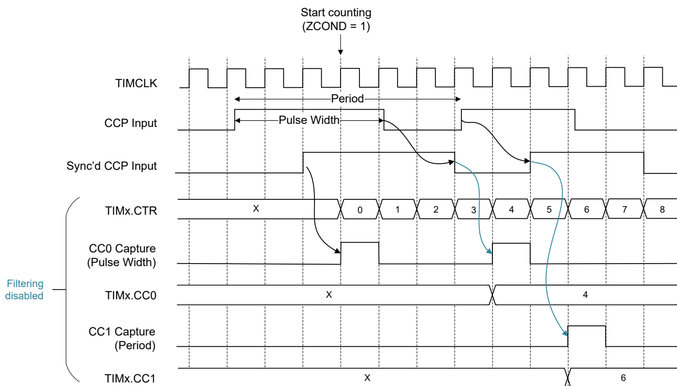
Figure 17-17. Combined Pulse-Width and Period Capture
