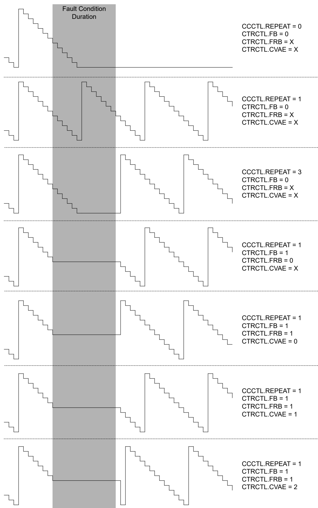
Figure 17-37. Counter Behavior in Fault Condition with TIMx.CTRCTL Register
