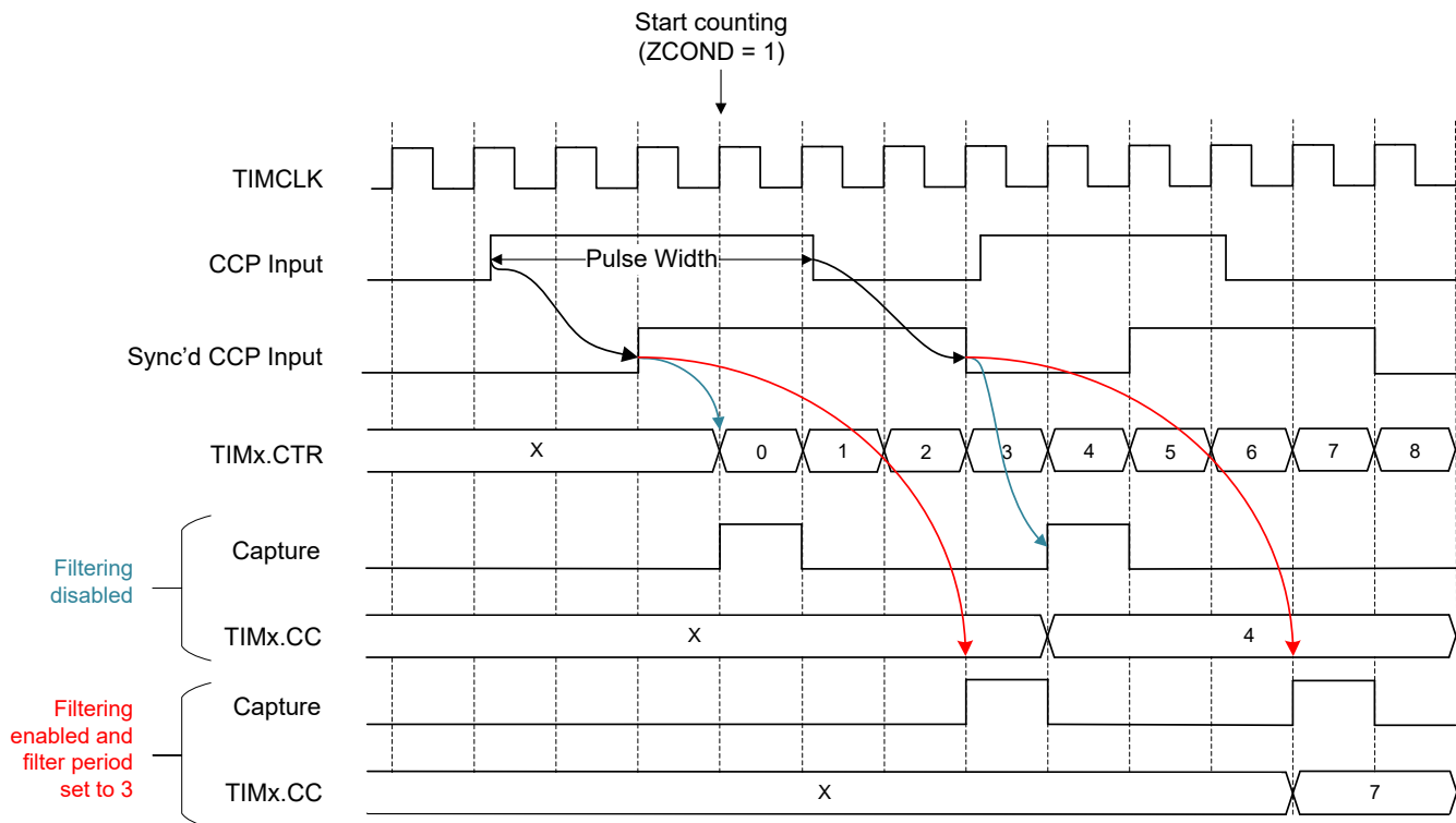
Figure 17-16. Pulse-Width Capture Mode
