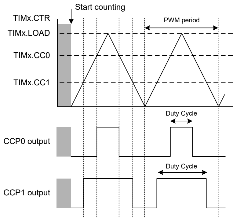
Figure 17-30. Center-Aligned PWM
