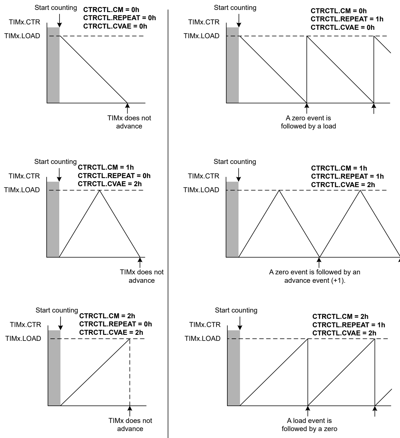
Figure 17-4. One-shot and Periodic Mode Behavior
