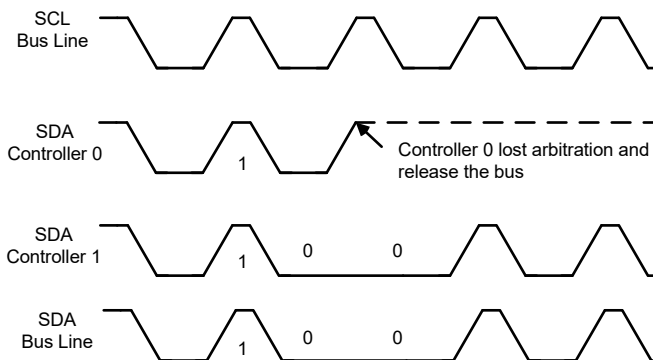
Figure 14-11. Arbitration Procedure Between Two Controller Transmitters
