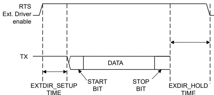
Figure 12-12. RS485 External Control
