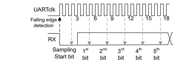
Figure 12-3. UART Oversampling mode
