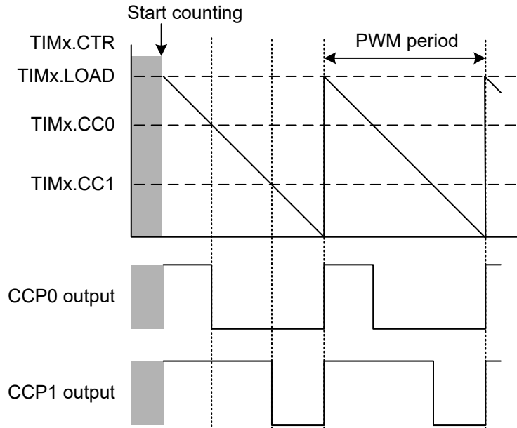
Figure 17-28. Edge-Aligned PWM Signals in Down-Counting Mode
