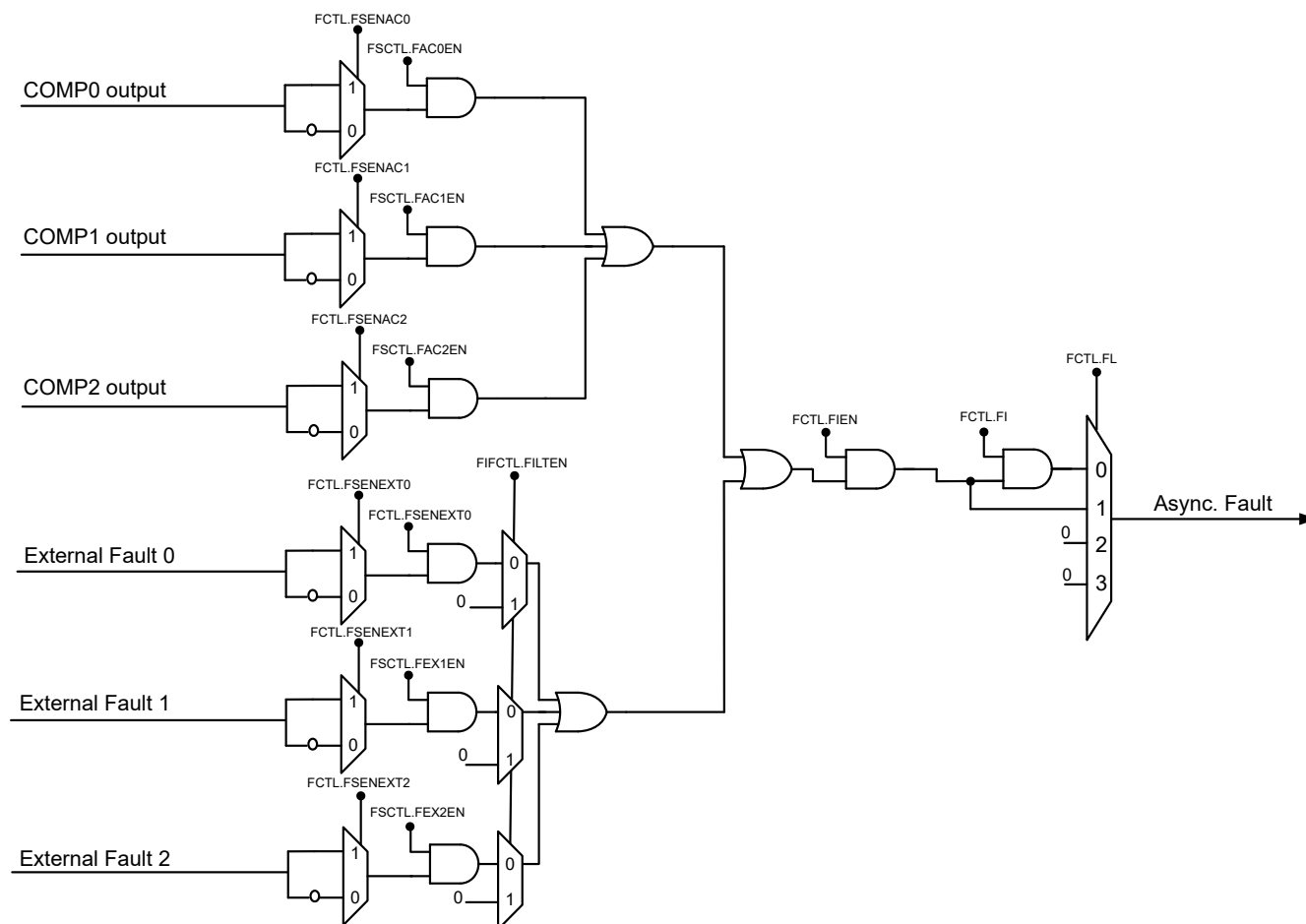
Figure 17-34. Asynchronous Fault Handler Connections
