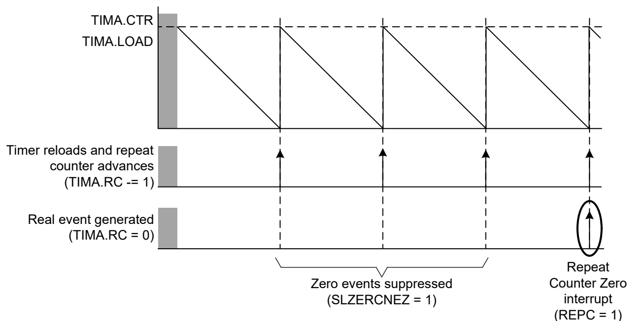
Figure 17-3. Event Suppressed by Repeat Counter with TIMx.RCLD = 4 in Down Counting Mode
