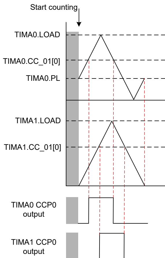
Figure 17-31. Asymmetric PWM Configuration with Phase Load for CCP channel 0 of TIMA0 and TIMA1
