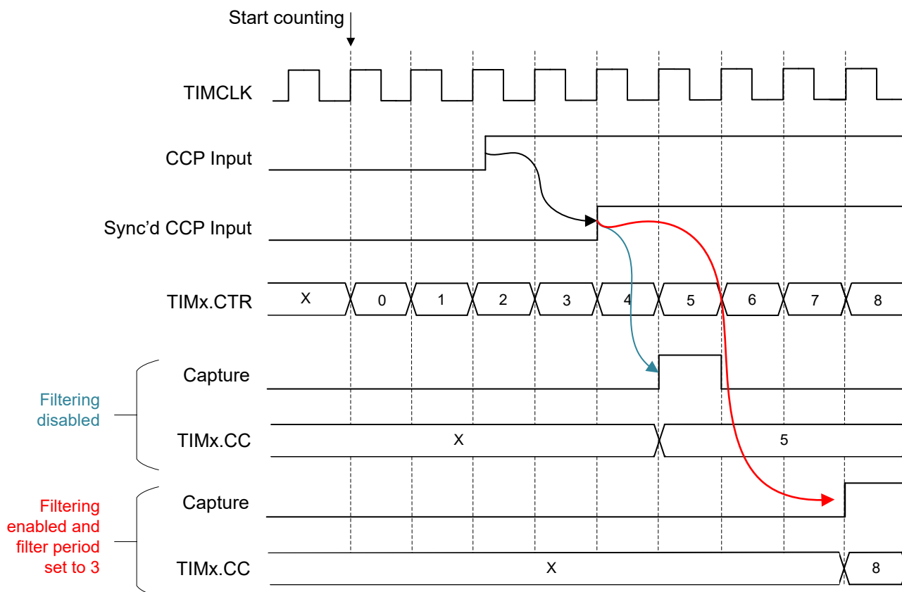
Figure 17-14. Edge Time Capture Mode in Up-Counting Mode, CVAE = 2
