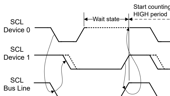
Figure 14-12. Clock Synchronization
