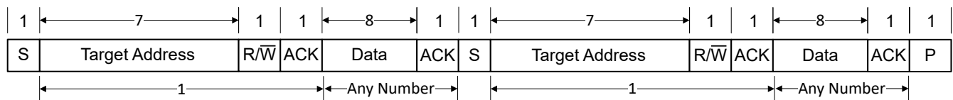
Figure 14-10. Data Format with Repeated Start
