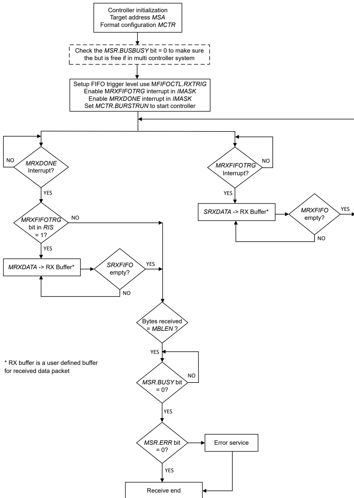
Figure 14-14. Controller Receiver Mode
