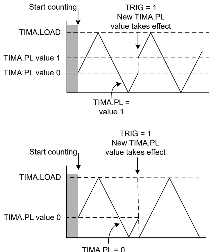
Figure 17-11. Phase Load Register Synchronization in Up-Down Mode
