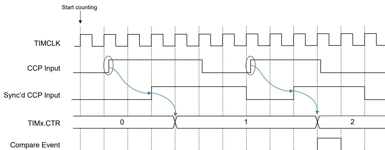
Figure 17-23. Edge Count Operation to Generate Compare Event (TIMx.CC = 2)
