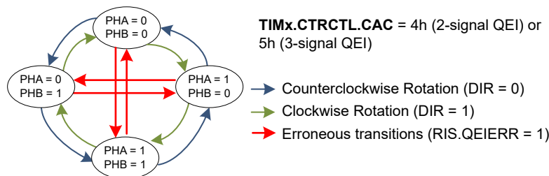
Figure 17-18. State Machine for 2-signal and 3-signal QEI mode
