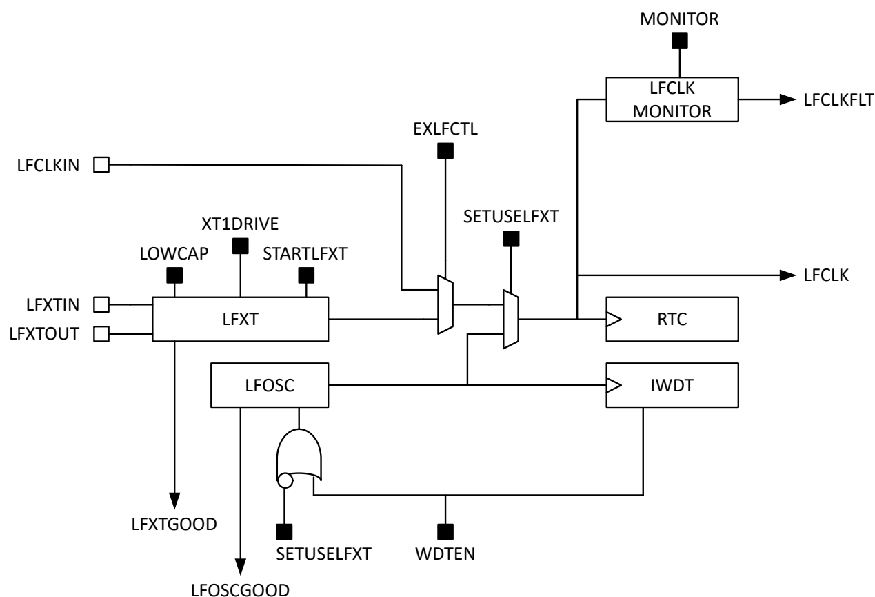
Figure 18-1. LFSS Low-Frequency Clock System
