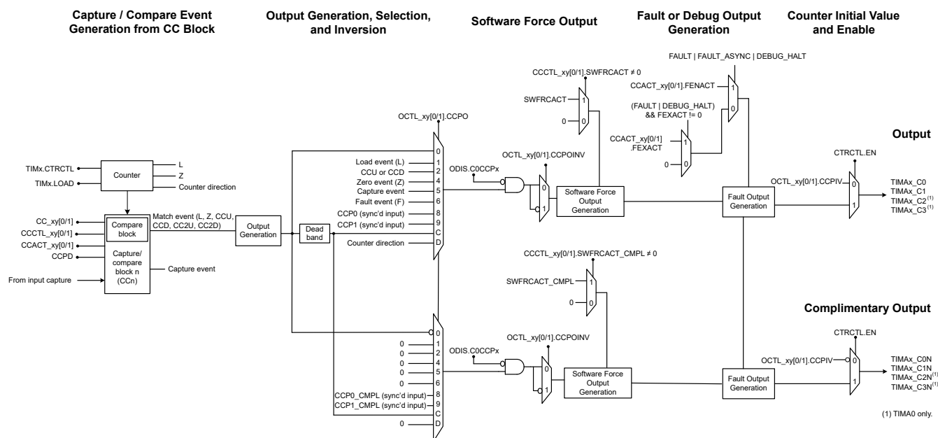
Figure 17-27. Output Connection for TIMA
