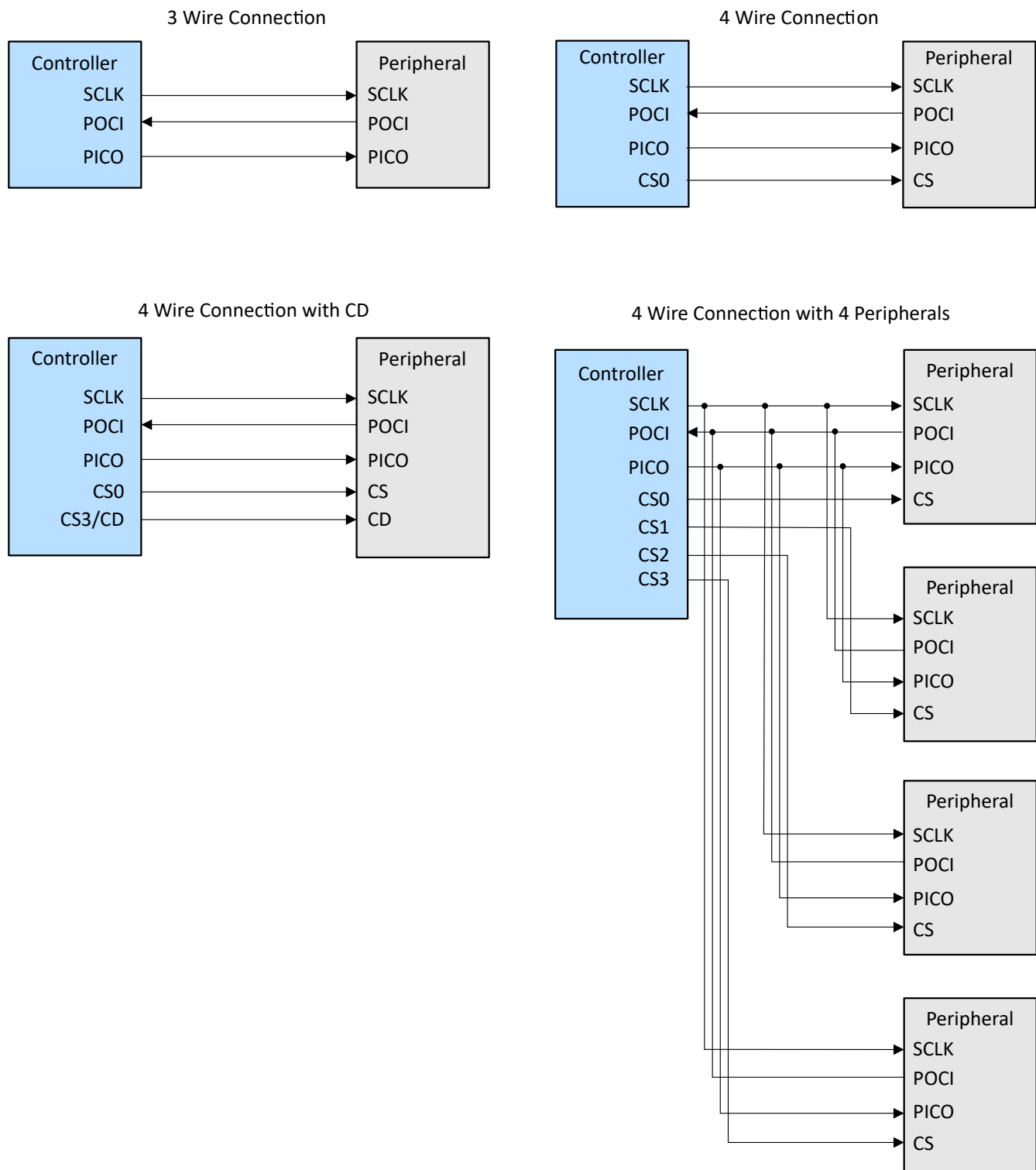
Figure 13-2. External Connections for Different SPI Configurations
