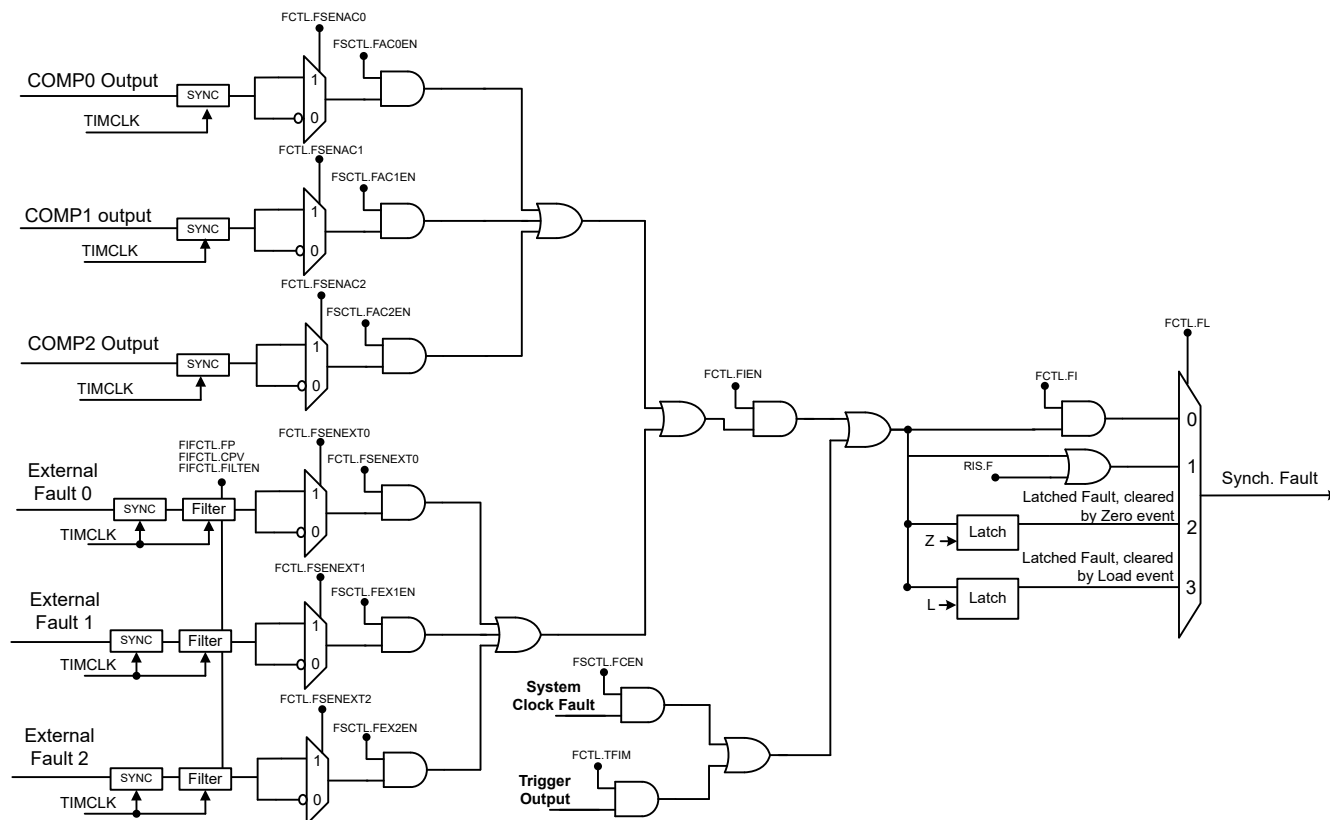
Figure 17-35. Synchronous Fault Handler Connections
