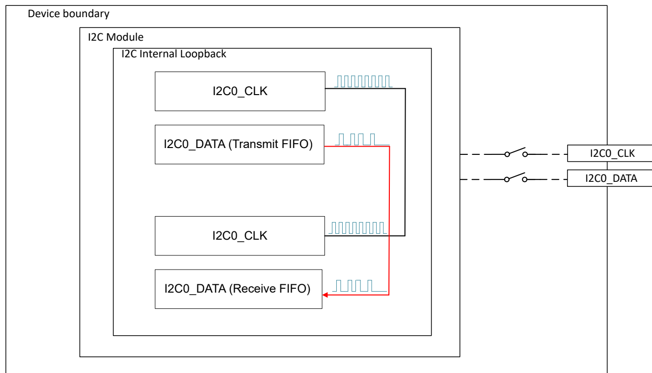
Figure 14-13. I2C Internal Loopback mode
