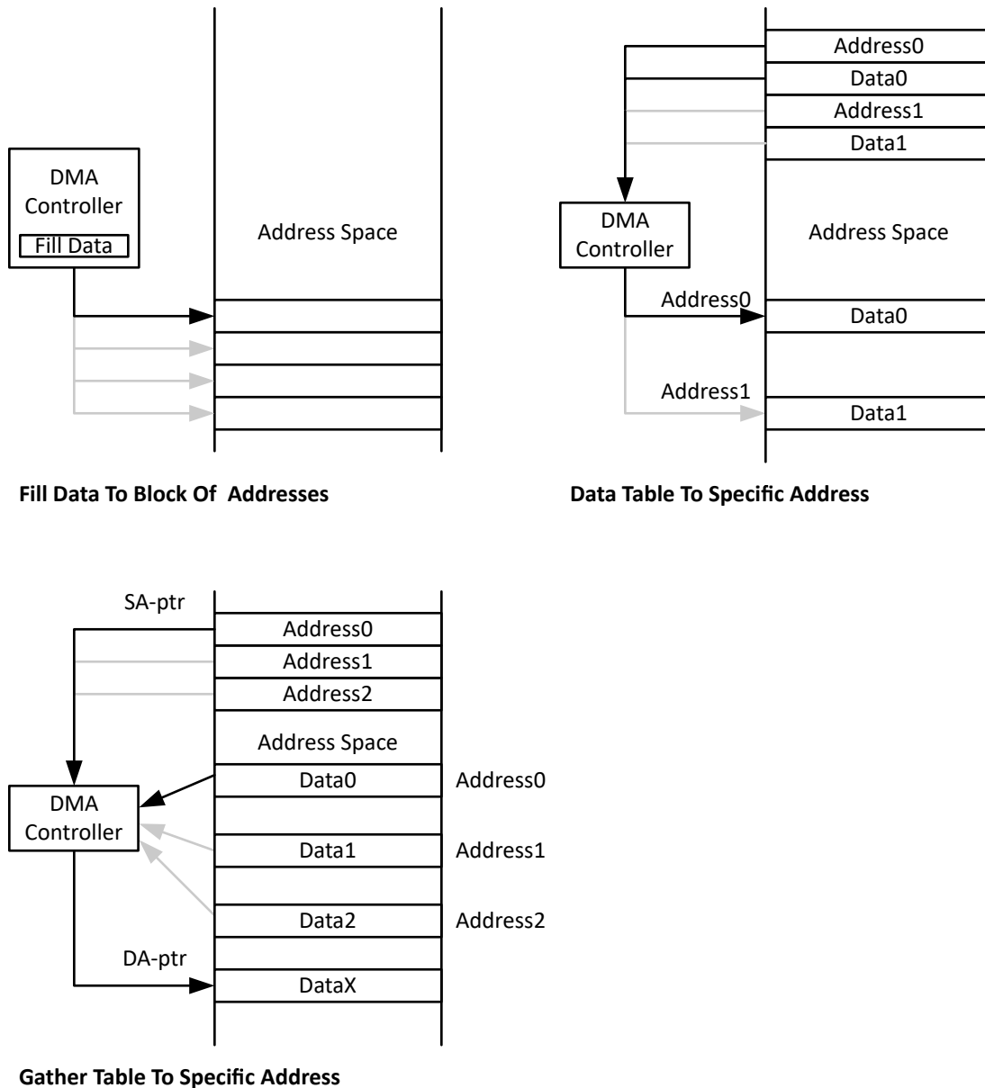
Figure 5-3. DMA Extended Modes Diagram
