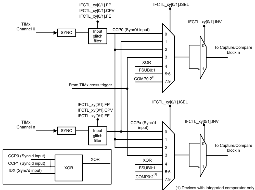
Figure 17-12. TIMx Capture Block Diagram
