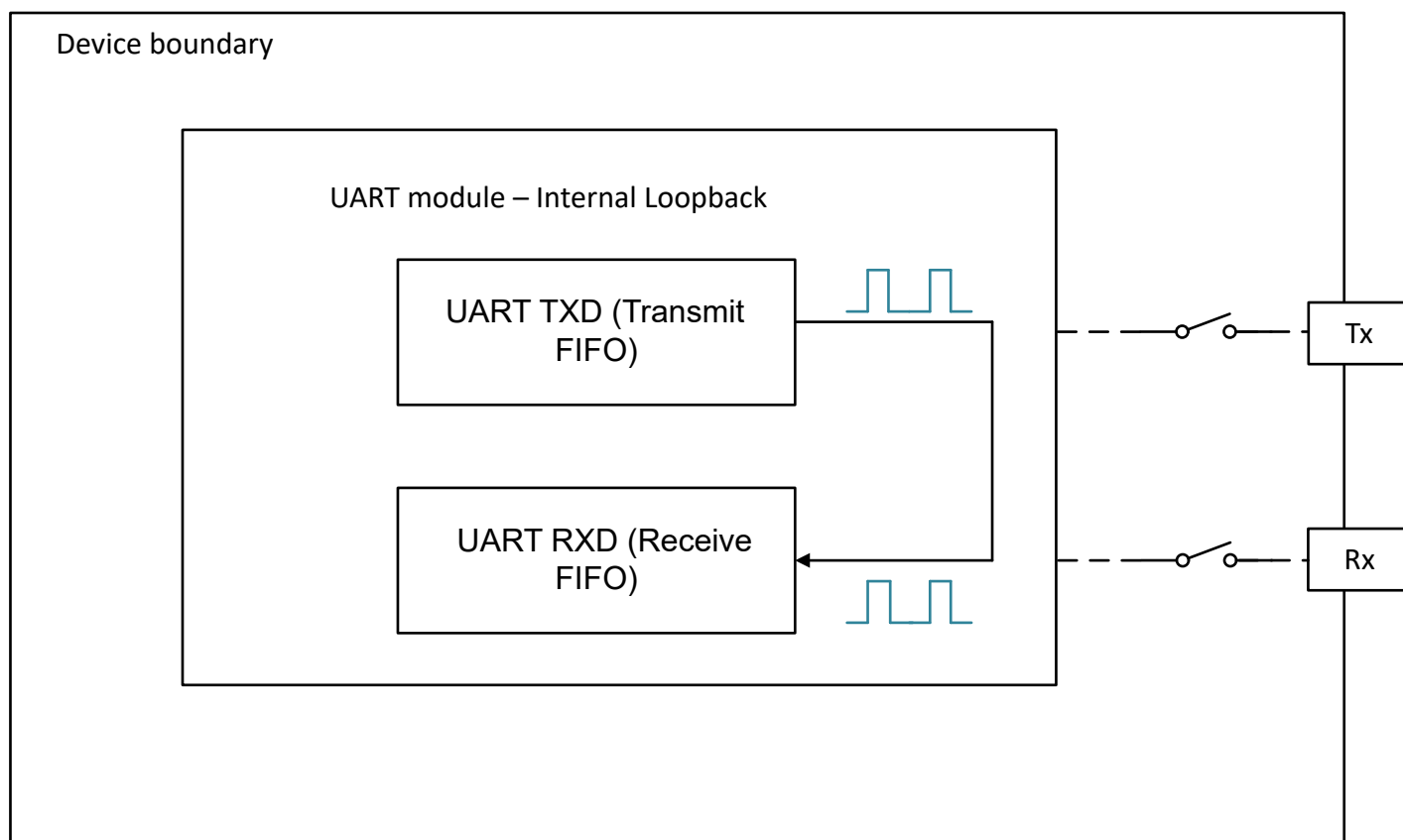
Figure 12-15. UART Loopback Mode
