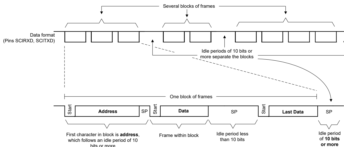
Figure 12-10. Idle-Line Multiprocessor
