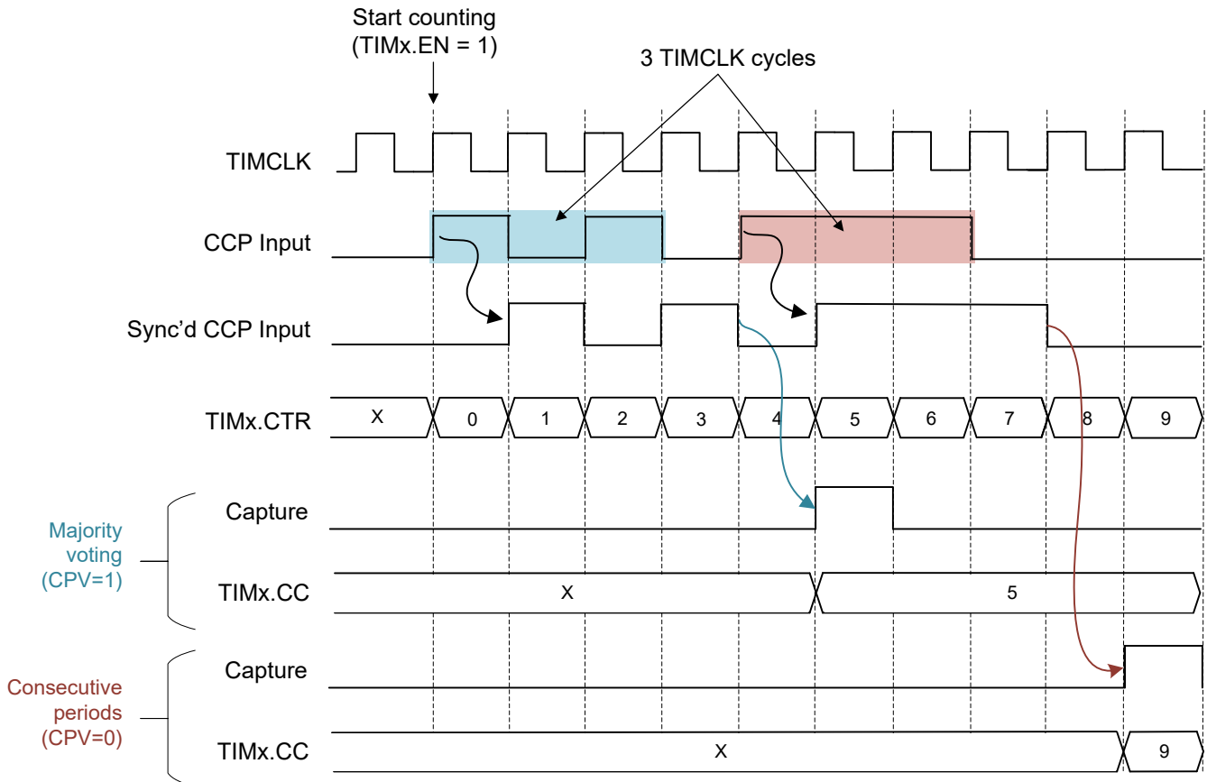
Figure 17-13. Consecutive Period and Majority Voting for Input Glitch Filtering using FP = 0 (3 TIMCLK cycles)
