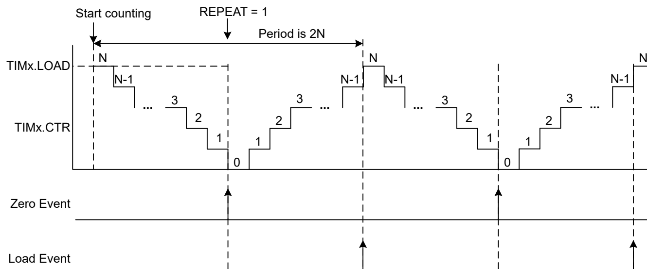
Figure 17-7. Down-up Counting Mode and Event Generation, CVAE = 0
