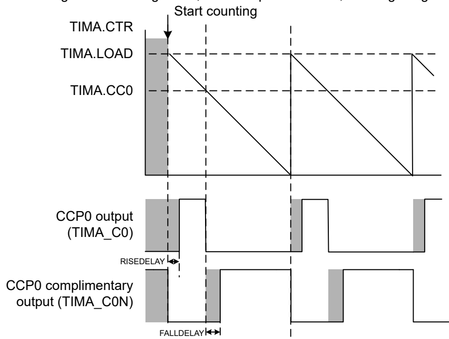
Figure 17-32. Deadband Insertion (Mode 0) for PWM in Down-Counting Mode
