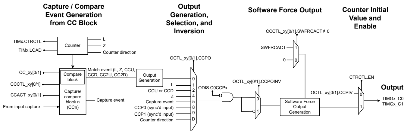
Figure 17-26. Output Connection for TIMG
