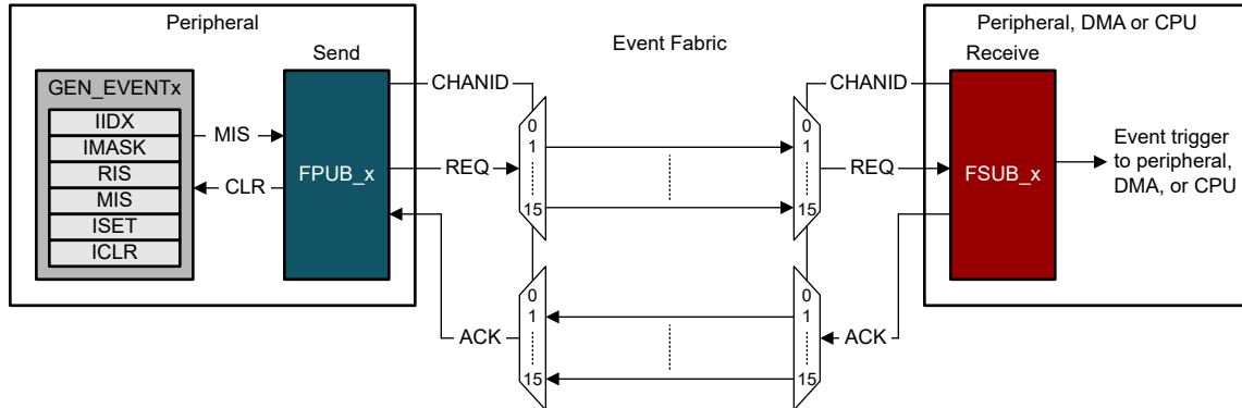
Figure 7-4. Generic Route
