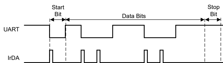
Figure 12-14. IrDA Protocol
