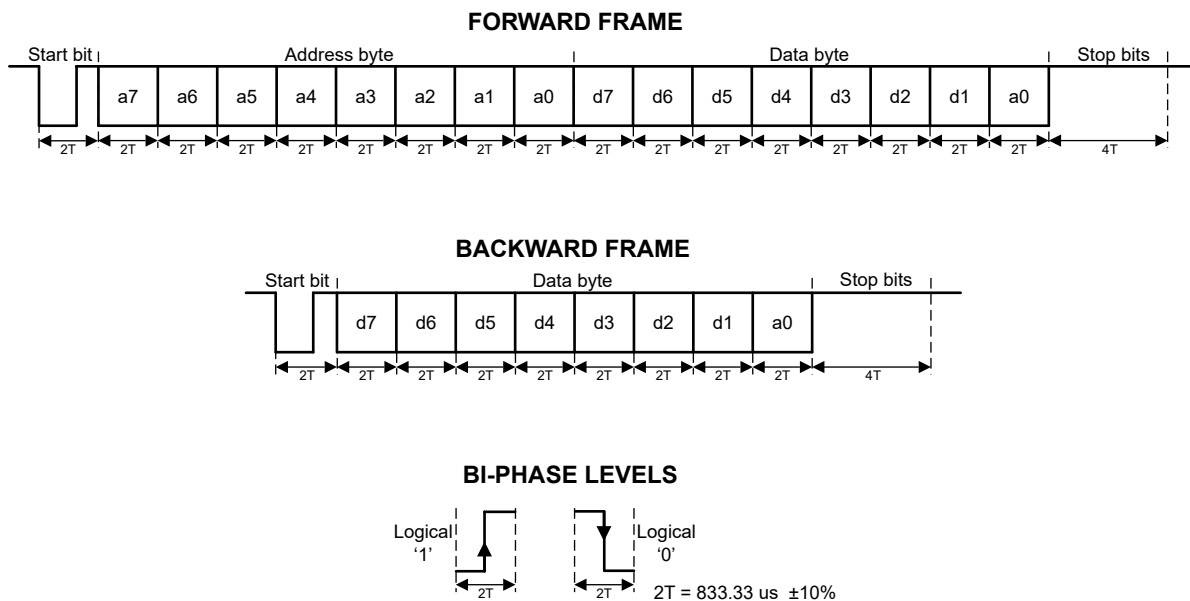
Figure 12-13. DALI Protocol
