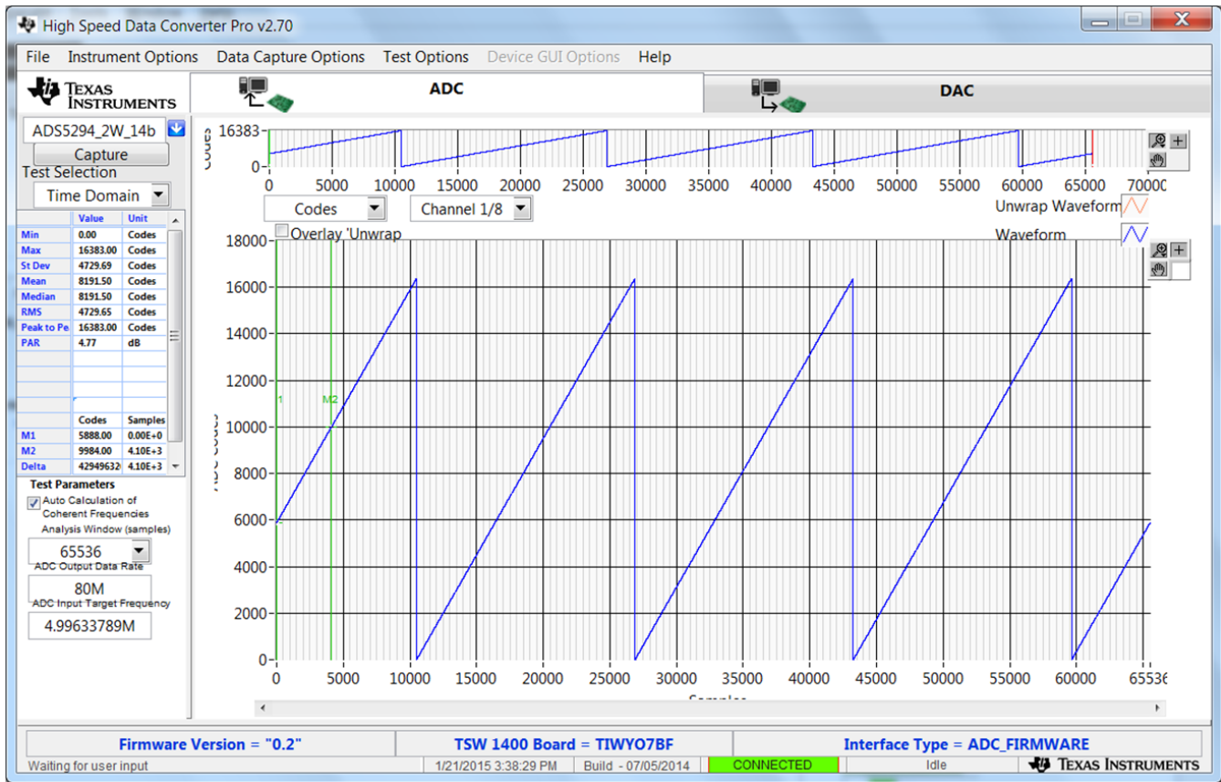
Figure 9. User Interface: Time Domain Format
