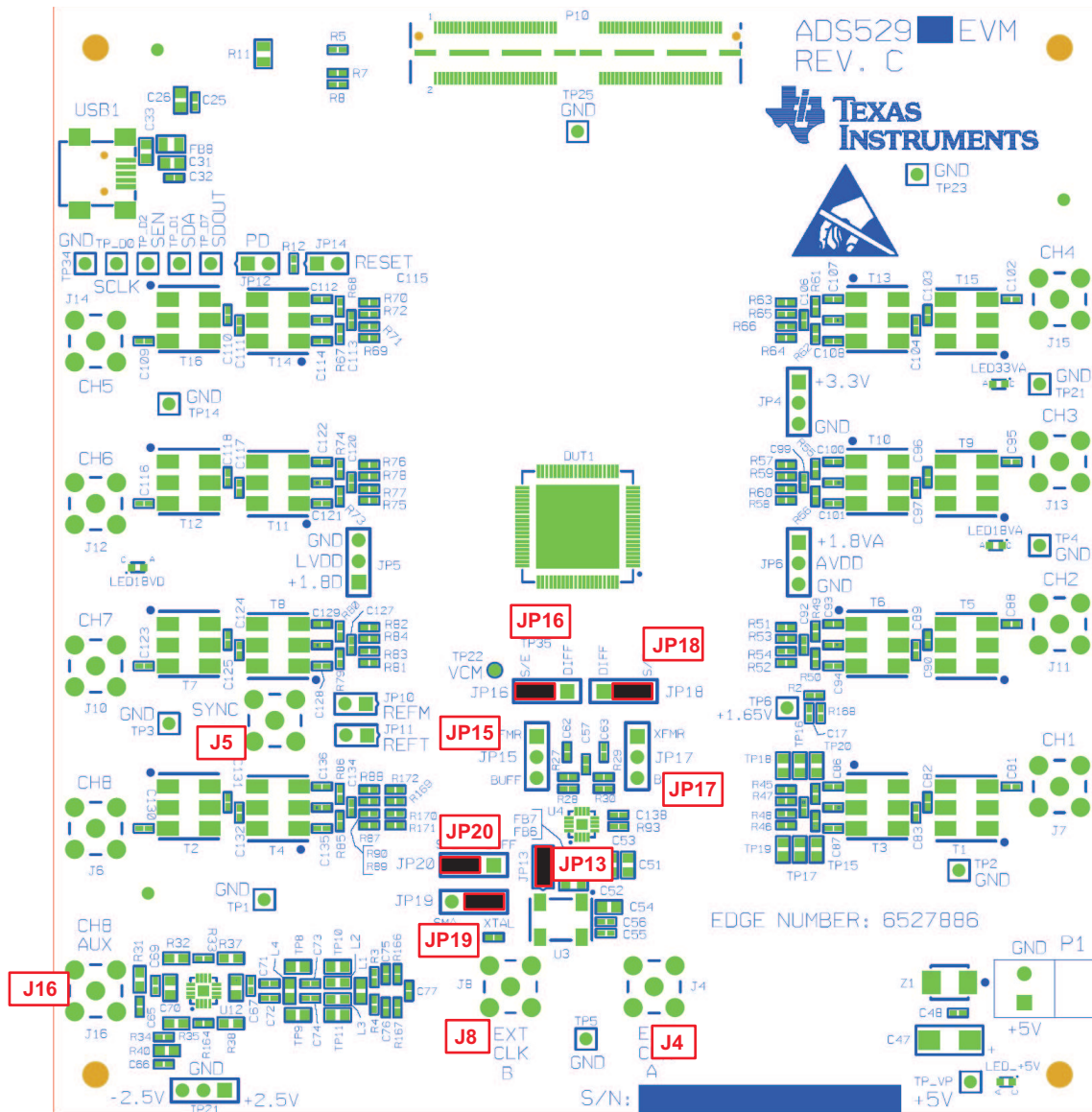
Figure 12. ADS5294EVM Default Clock Jumper Locations
