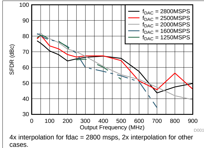
Figure 7. SFDR vs Output Frequency Over f_{\text{DAC}}
