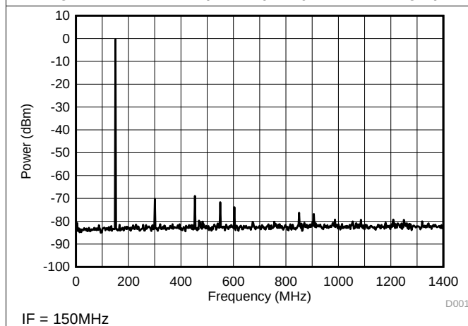
Figure 11. Single Tone Spectral Plot
