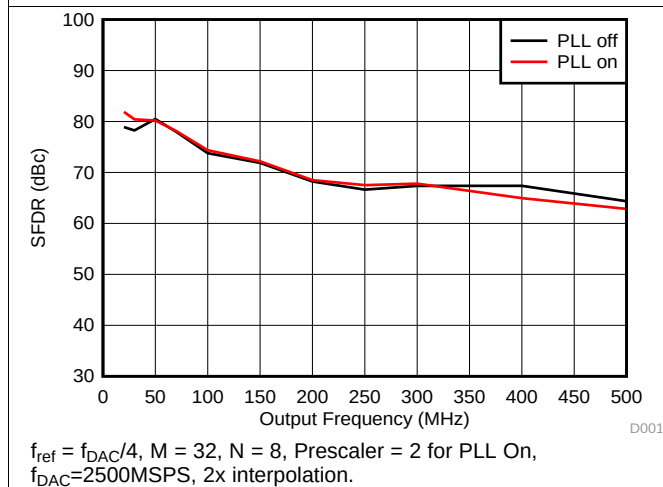
Figure 9. SFDR vs Output Frequency Over Clocking Options
