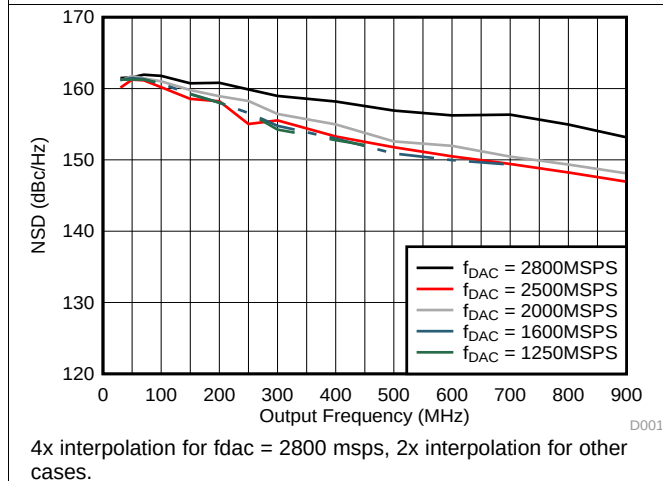
Figure 23. NSD vs Output Frequency Over f_{DAC}
