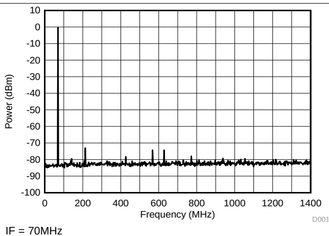
Figure 10. Single Tone Spectral Plot
