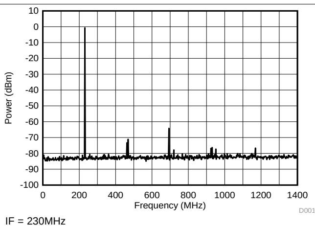
Figure 12. Single Tone Spectral Plot
