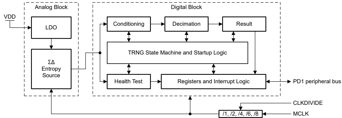
Figure 5-1. TRNG Block Diagram
