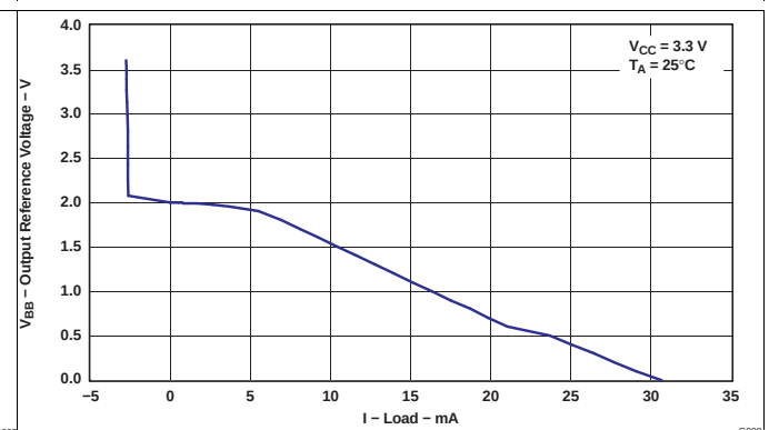
Figure 9. Output Reference Voltage (VBB) vs Load
