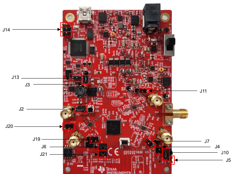
Figure 3-2. Jumper Locations
