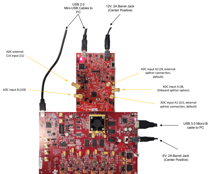
Figure 3-1. TRF1305-ADC32RFEVM Bench Setup Block Diagram
