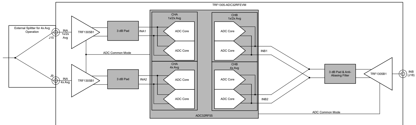
Figure 3-14. Analog Input Configuration
