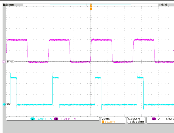
IOUT = 1 A f (SYNC) = 2 MHz Figure 9-31. Synchronization to an External Clock
