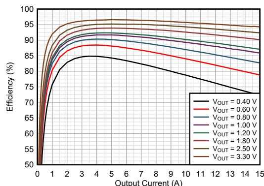
Efficiency TPSM8287A15BAH (V IN = 5.0V; FPWM)
