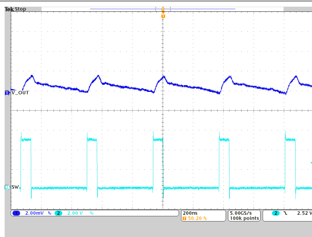
Vout = 0.9 V IOUT = 2 A Figure 9-27. PWM-CCM Operation TPSM8287A12BBS
