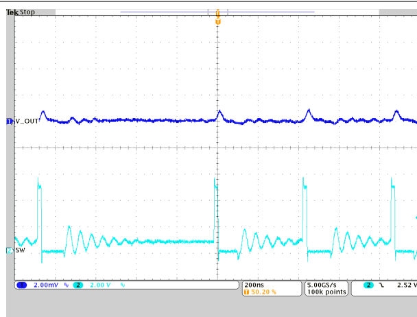
Vout = 0.9 V IOUT = 100 mA Figure 9-29. PFM-DCM Operation TPSM8287A12BBS
