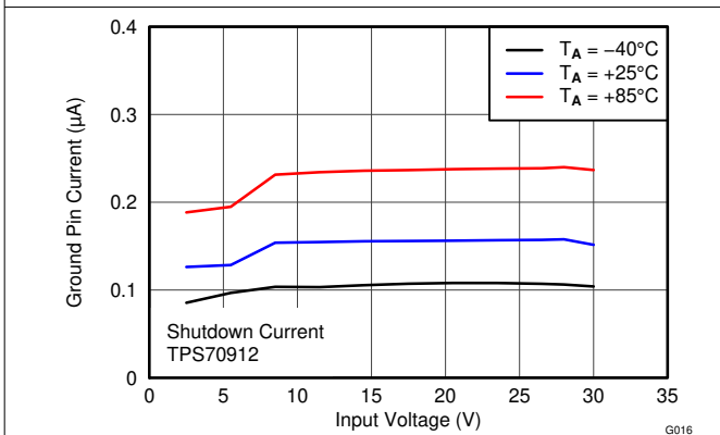
Figure 6-15. GND Current vs V_{IN} and Temperature
