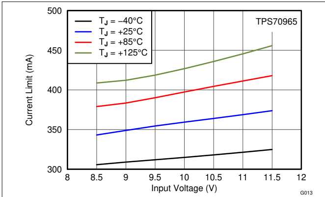
Figure 6-13. 6.5-V Current Limit vs V_{IN} and Temperature
