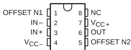
JG PACKAGE (TOP VIEW)
