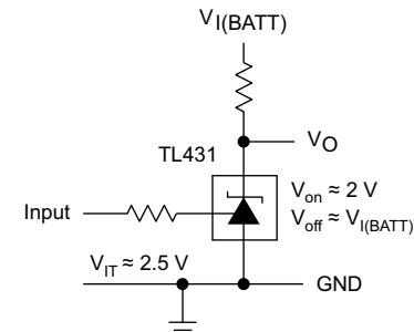
Figure 29. Single-Supply Comparator with Temperature-Compensated Threshold
