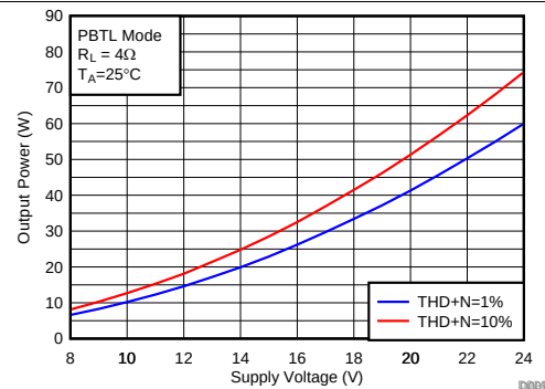
Figure 41. Power vs Supply Voltage (PBTL Mode)
