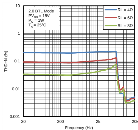
Figure 23. Total Harmonic Distortion vs Frequency
