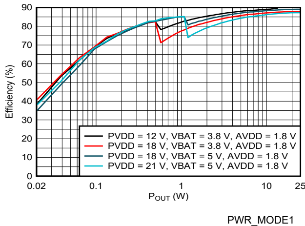
Figure 9-4. Efficiency vs Output Power
