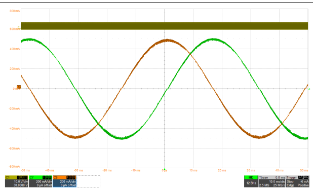
Figure 8-12. 1/256 Microstepping With smart tune Dynamic Decay
