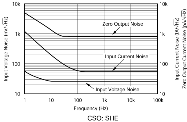
Figure 5-15. Input Voltage, Input Current, and Zero Output Current Noise Density vs Frequency
