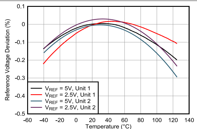
Figure 5-24. Reference Voltage Deviation vs Temperature
