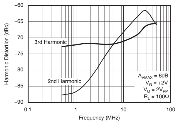
Figure 16. Harmonic Distortion vs Frequency
