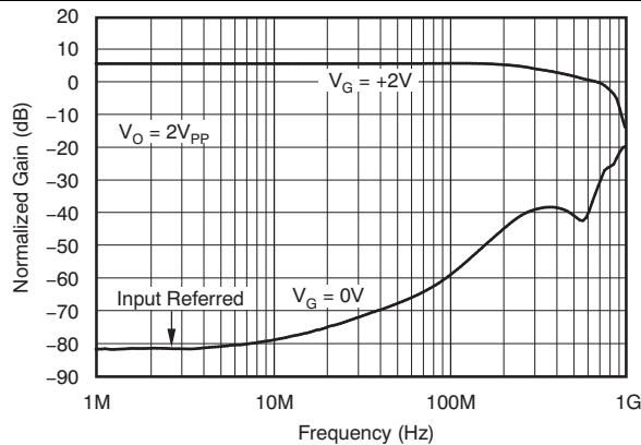
Figure 25. Fully-Attenuated Response
