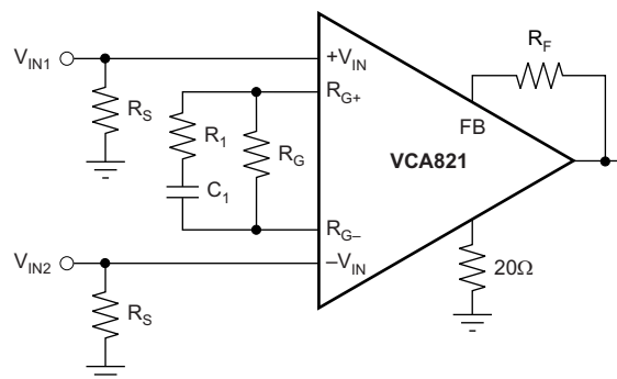
Figure 83. Differential Equalizer
