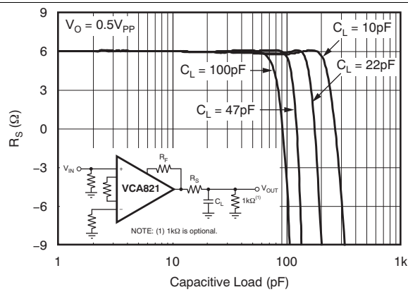
Figure 29. Frequency Response vs Capacitive Load
