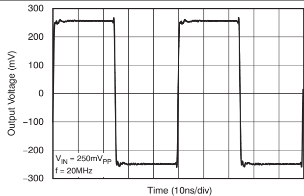
Figure 12. Small-Signal Pulse Response
