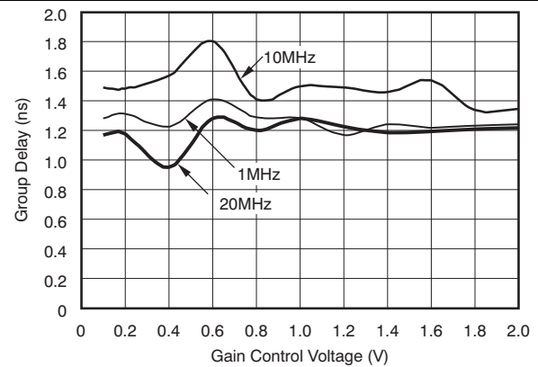
Figure 26. Group Delay vs Gain Control Voltage
