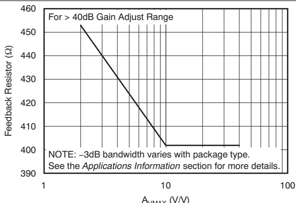
Figure 6. Recommended R_F vs A_{V\text{MAX}}
