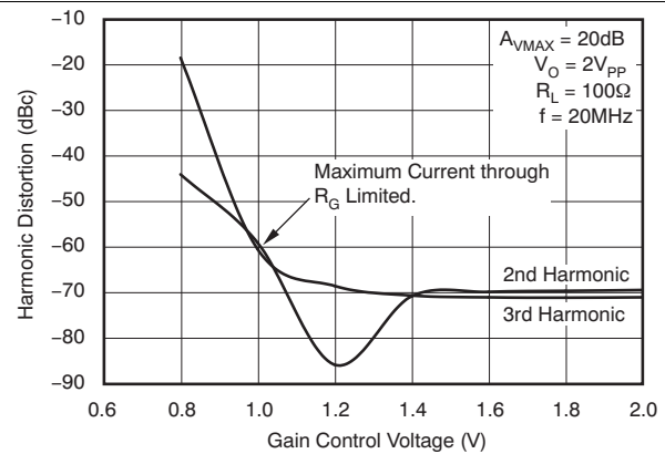
Figure 41. Harmonic Distortion vs Gain Control Voltage
