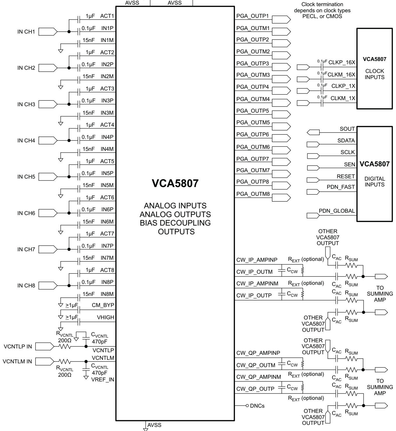
Figure 81. Application Circuit
