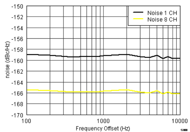
Figure 17. CW Thermal Noise 1-CH vs 8-CHs
