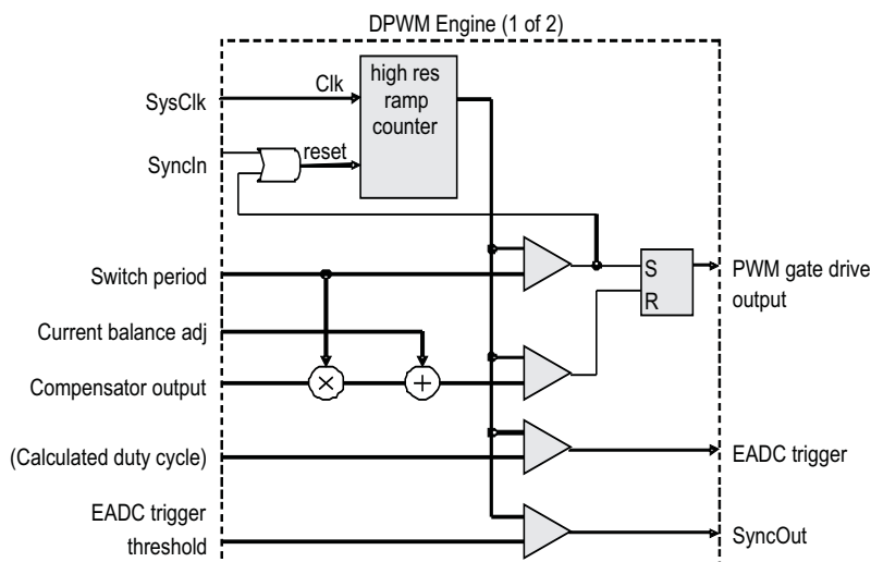
Figure 12. DPWM Engine
