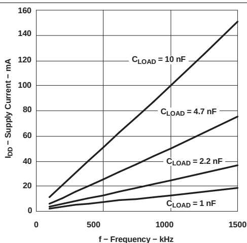
Figure 5. Supply Current vs Frequency ( V_{DD} = 5\text{ V} )
