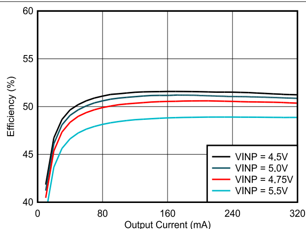
Figure 6-7. Efficiency vs Load Current (Ivcc): VCC = 3.3V, TA = 25°C, COUT2 = 22µF
