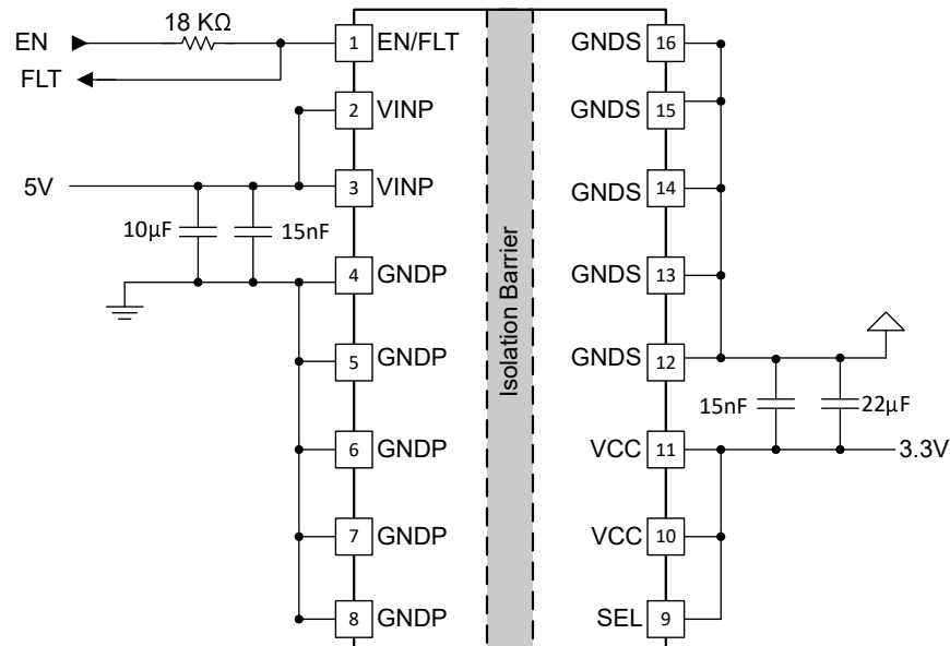
Figure 8-1. Typical Application
