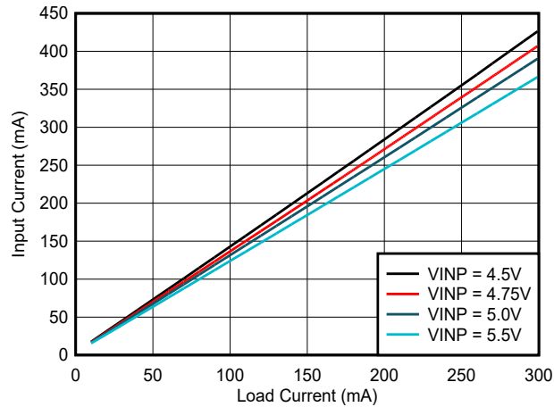
Figure 6-11. Input Current ( I_{VINP} ) vs Load Current ( I_{VCC} ): V_{CC} = 3.3V , T_A = 25^\circ C , C_{OUT2} = 22\mu F
