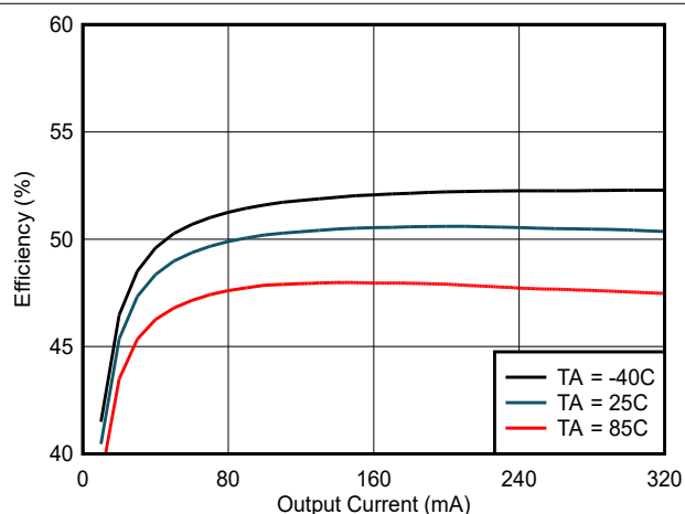
Figure 6-8. Efficiency vs Load Current (Ivcc): VCC = 3.3V, VINP = 5.0V, COUT2 = 22µF
