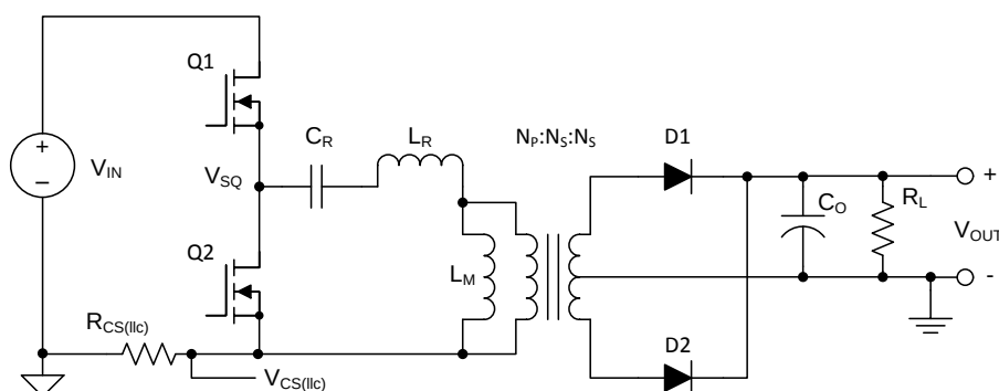
Figure 29. Basic LLC Schematic
