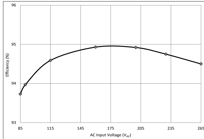
Figure 42. Full-Load Efficiency in Universal AC Line
