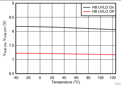
Figure 14. VHB-VHS UVLO Thresholds vs Temperature
