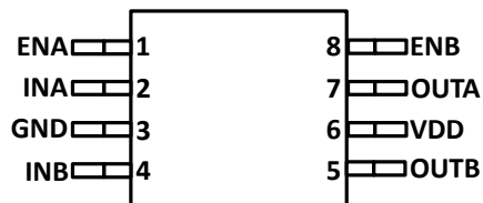
Figure 4-3. DGK Package 8-Pin VSSOP Top View
