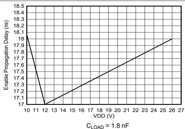
Figure 5-20. Enable to Output Rising Propagation Delay
