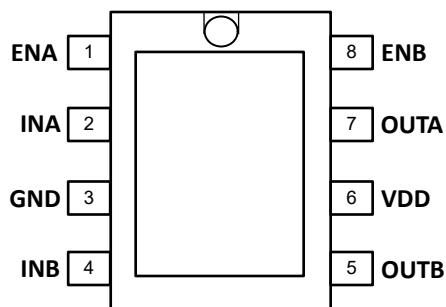
Figure 4-4. DDA Package 8-Pin SOIC Top View
