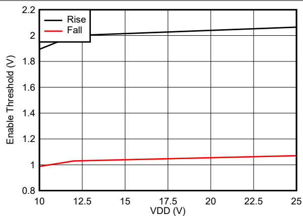
Figure 5-10. Enable Threshold
