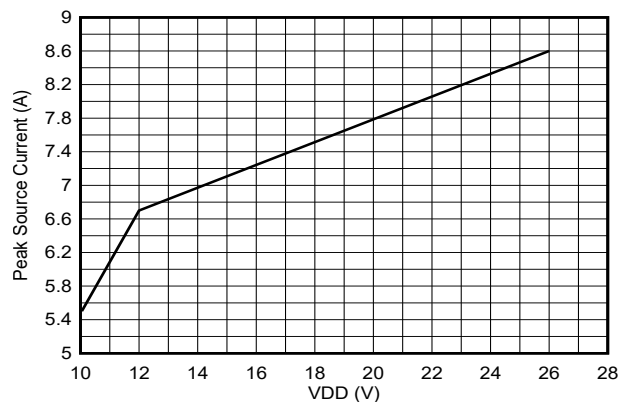
Figure 5-24. Peak Source Current vs VDD
