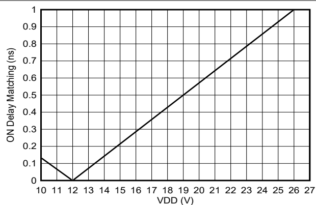
Figure 5-22. Turn-On/Rising Delay Matching
