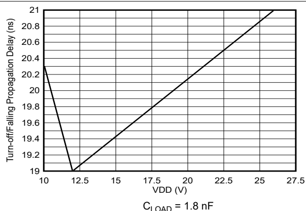
Figure 5-18. Input to Output Falling (turn-off) Propagation Delay vs VDD
