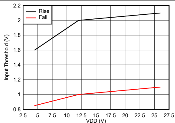
Figure 5-8. Input Thresholds
