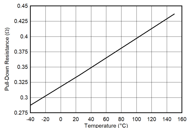
Figure 6-19. Output Pulldown Resistance vs VDD
