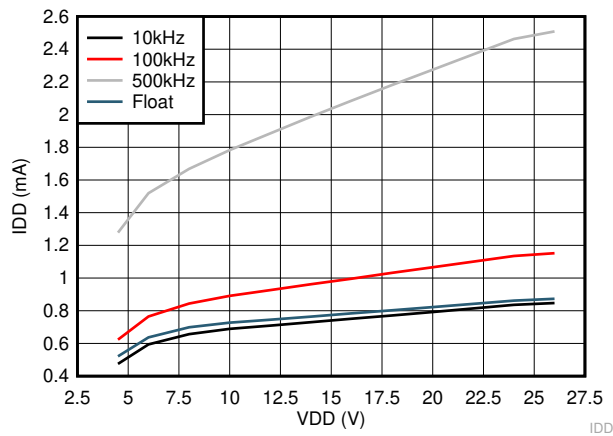
Figure 6-12. Operating Supply Current vs VDD
