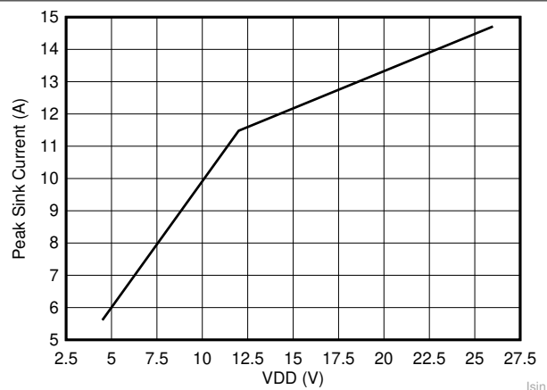
Figure 6-5. Peak Sink Current vs VDD
