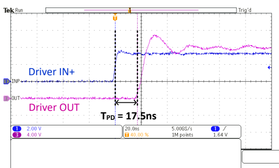
Figure 8-3. UCC27614 Rising (Turn-On) Propagation Delay
