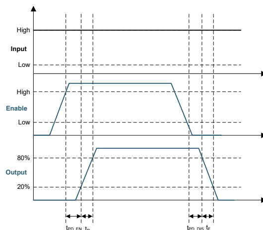
Figure 6-2. Enable Function
