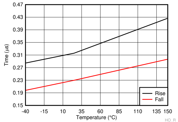
Figure 6-20. HO Fall Time
