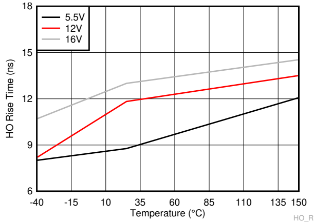
Figure 6-19. HO Rise Time
