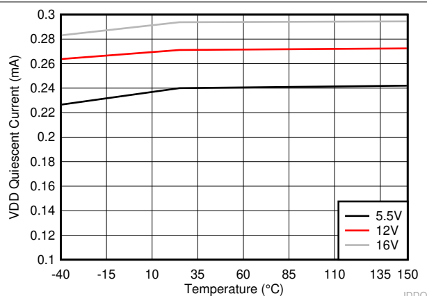
Figure 6-1. VDD Quiescent Current
