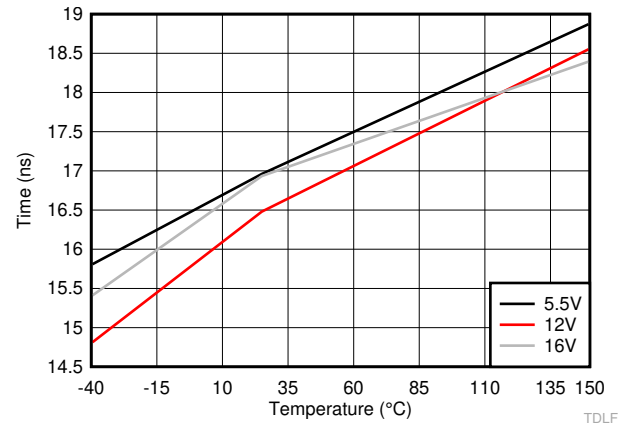
Figure 6-26. LO Falling Propagation Delay (TDLFF)
