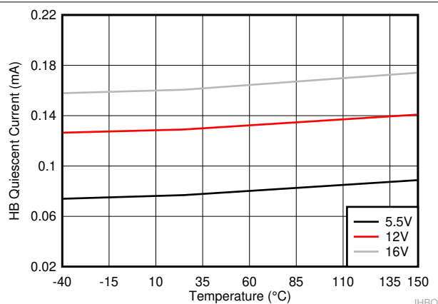
Figure 6-2. HB Quiescent Current
