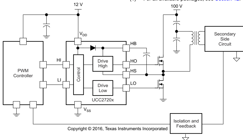
Simplified Application Diagram
