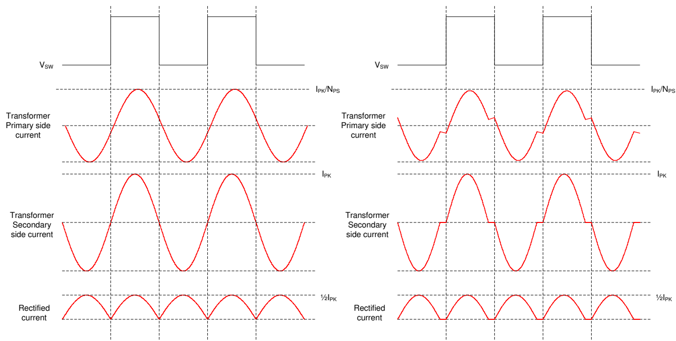
(a) Switching frequency equal to resonant frequency (b) Switching frequency below resonant frequency
