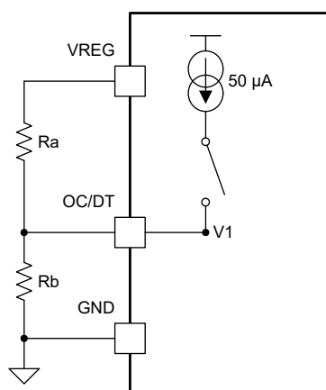
Figure 8-12. Current Source On
