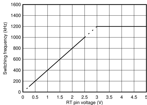
Figure 8-2. Relationship between switching frequency and RT-pin voltage
