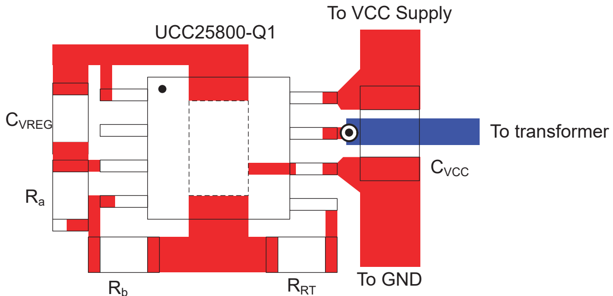
Figure 11-1. Layout example
