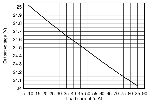
Figure 9-10. LLC output voltage load regulation
