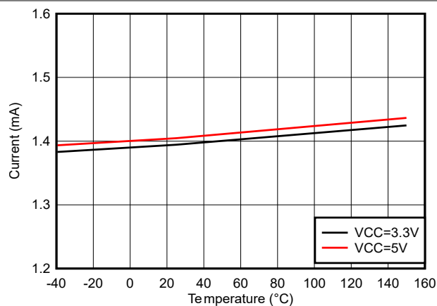
Figure 6-4. VCCI Quiescent Current
