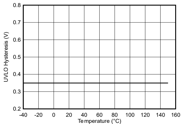
Figure 6-9. 5-V VDD UVLO Hysteresis Voltage
