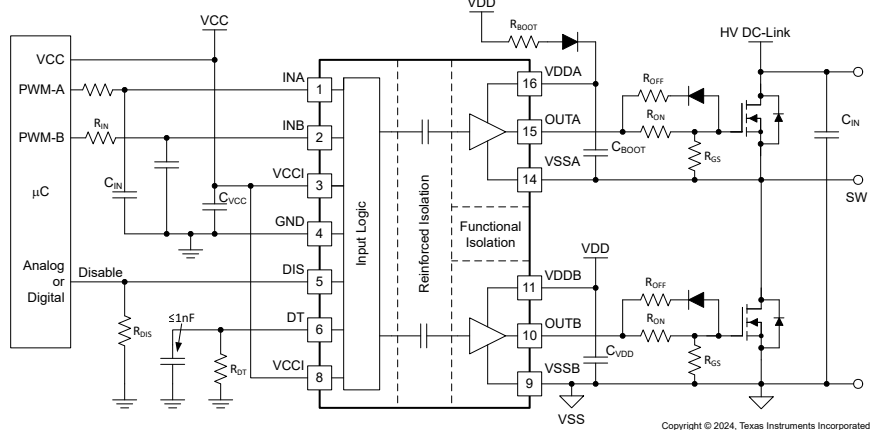
Typical Application
