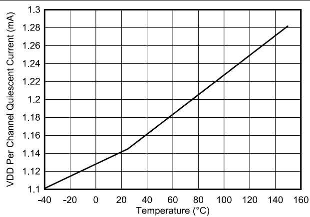
Figure 6-5. VDD Per Channel Quiescent Current ( I_{VDDA} , I_{VDDB} )
