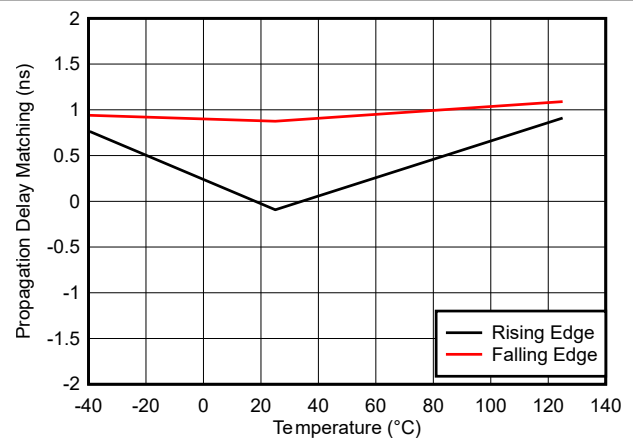
Figure 6-15. Propagation Delay Matching, Rising and Falling Edge
