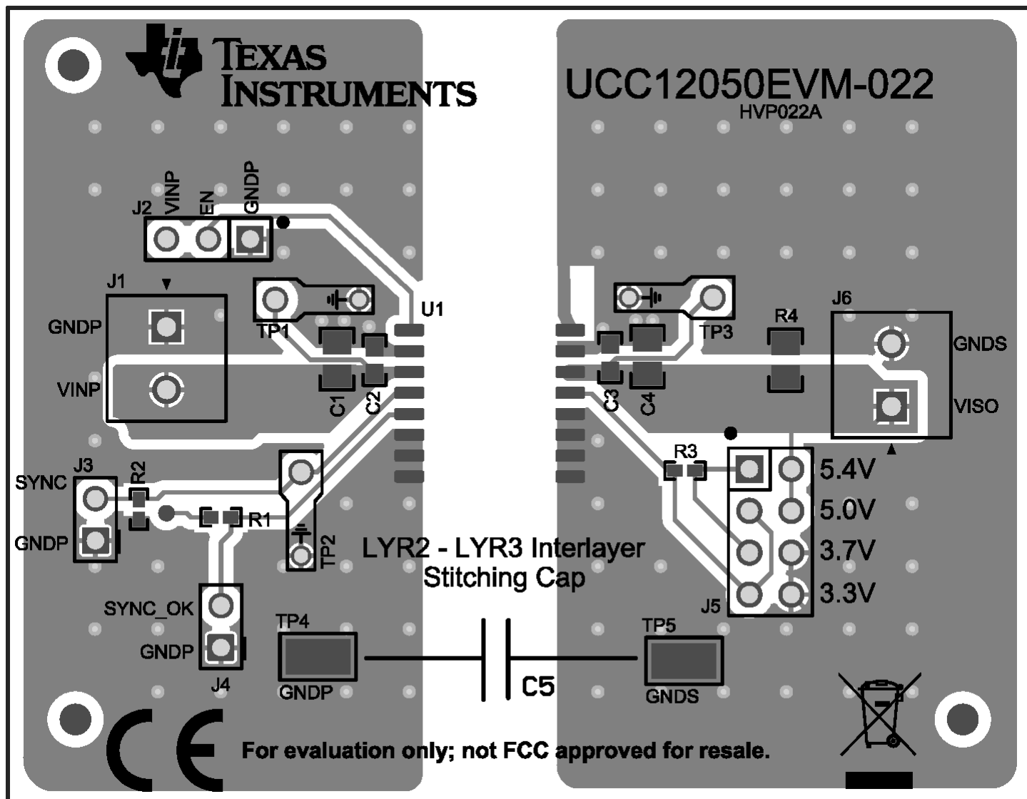
Figure 10-1. Layout Example
