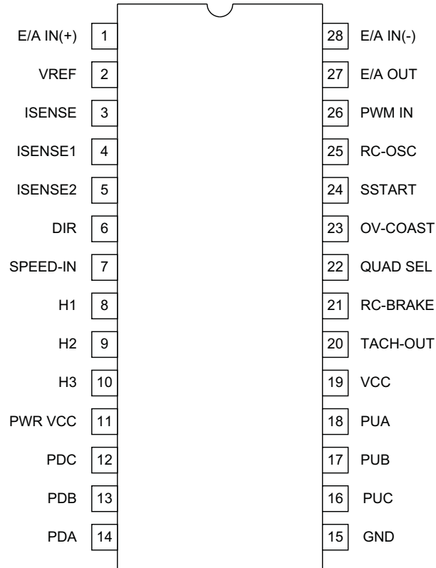
Figure 1. CONNECTION DIAGRAM
