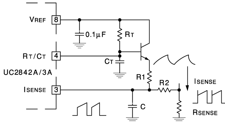
Figure 8-3. Slope Compression
