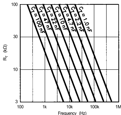
Figure 15. Timing Resistance vs Frequency
