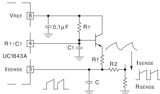
Figure 12. Current-Sense Circuit
