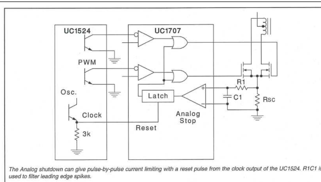
Figure 6. Current Limiting
