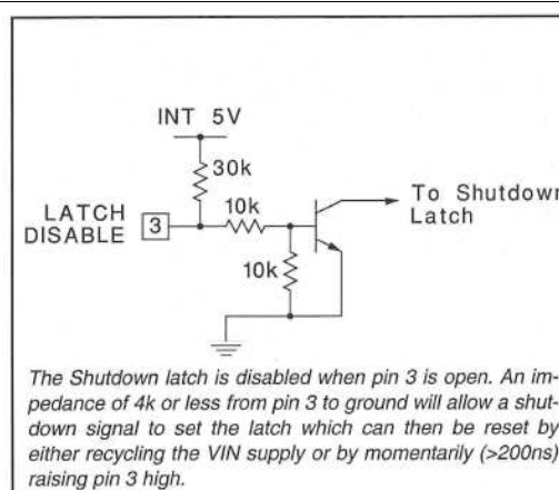
Figure 3. Latch Disable
