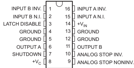
J or W Package 16-Pin CDIP or CFP Top View
