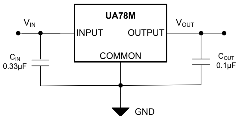
Figure 7-1. Fixed-Output Regulator
