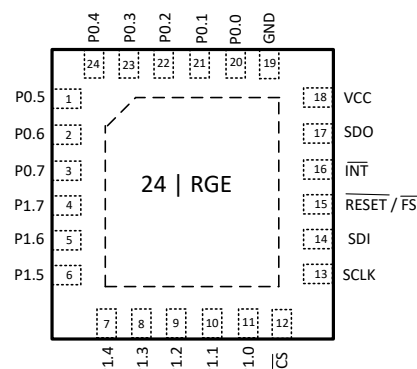
Figure 4-2. TXE8116-Q1 RGE (VQFN) Package, 24-Pin (Top View)
