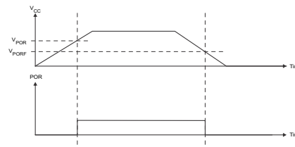
Figure 8-5. V_{POR}
