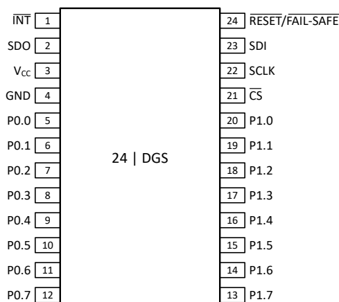
Figure 4-1. TXE8116-Q1 DGS (VSSOP) Package, 24-Pin (Top View)
