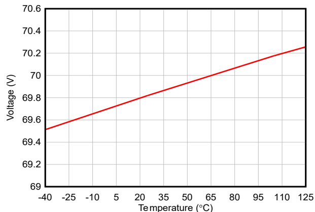
Figure 6-2. Breakdown Voltage (1mA) vs Temperature
