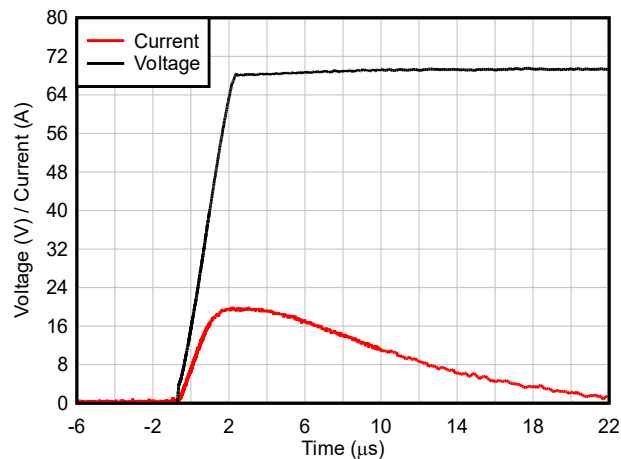
Figure 6-1. 8/20 \mu s Surge Response at 20A
