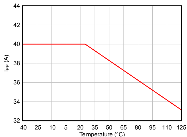
Figure 6-6. Max Surge Current (8/20 \mu s) vs Temperature
