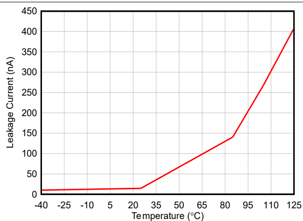
Figure 6-4. Leakage Current vs Temperature at 58V
