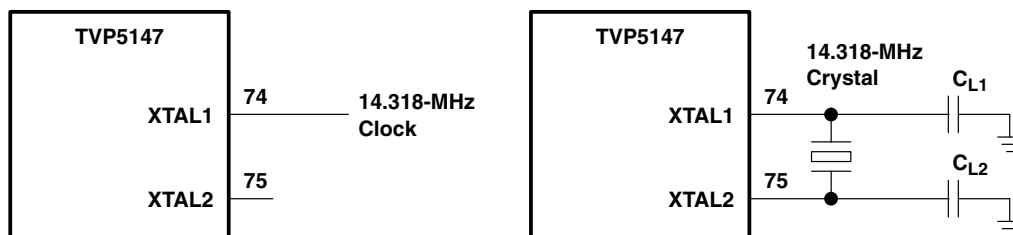
Figure 2-16. Reference Clock Configurations
