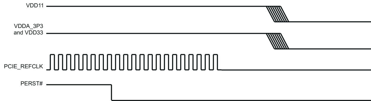
Figure 7-17. Power-Down Sequence
