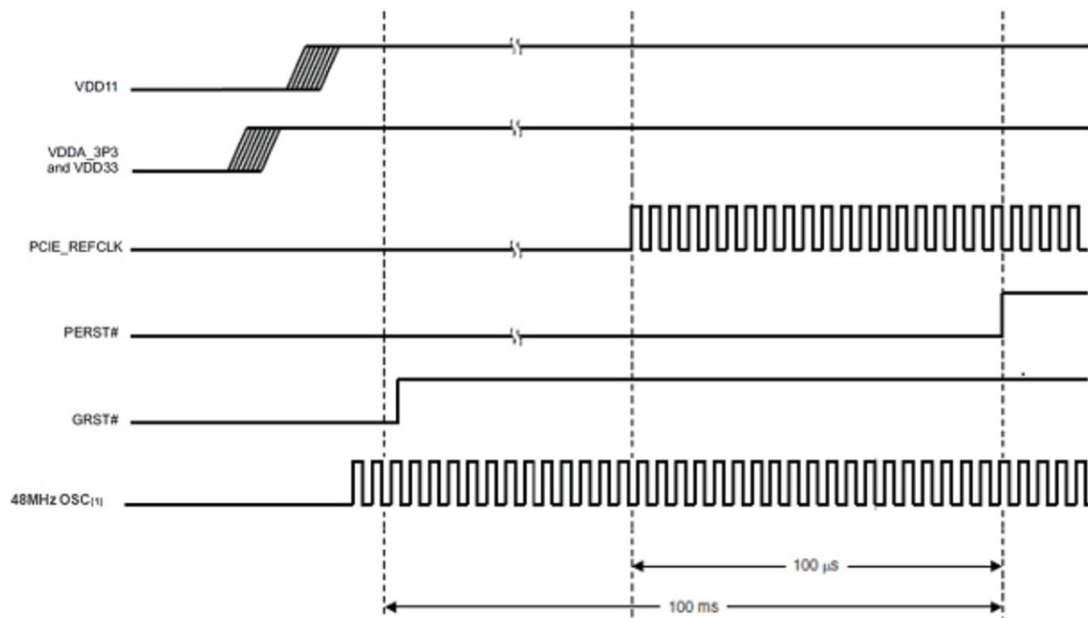
Figure 7-16. Power-Up Sequence
