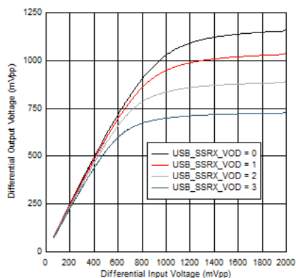
Figure 5-15. USB SSRX VOD Linearity Settings at 100MHz
