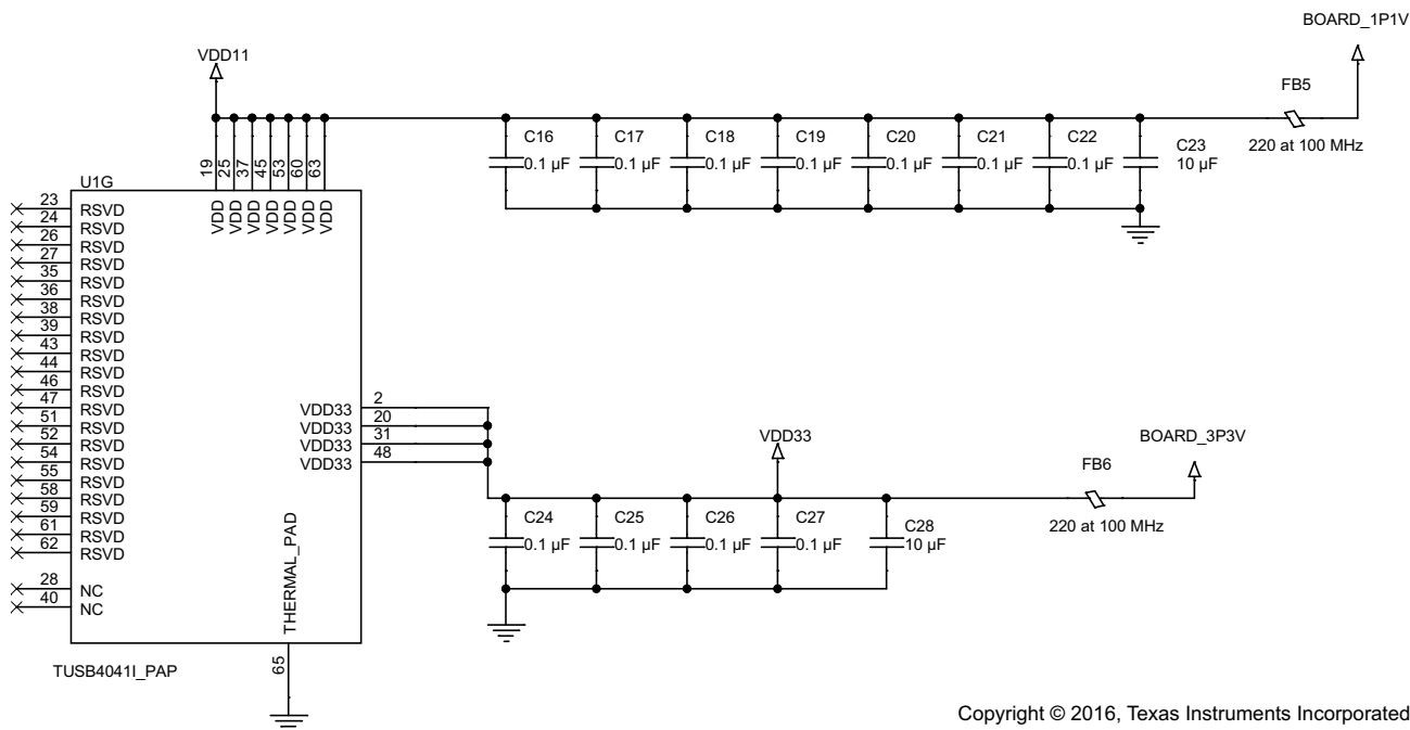
Figure 7-9. TUSB4041I Power Implementation
