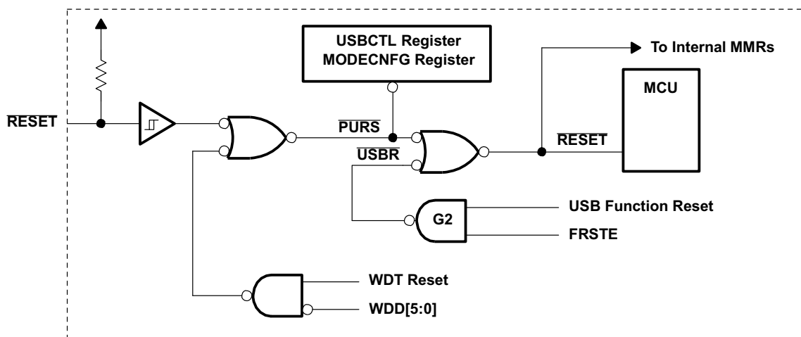
Figure 5-9. Reset Diagram
