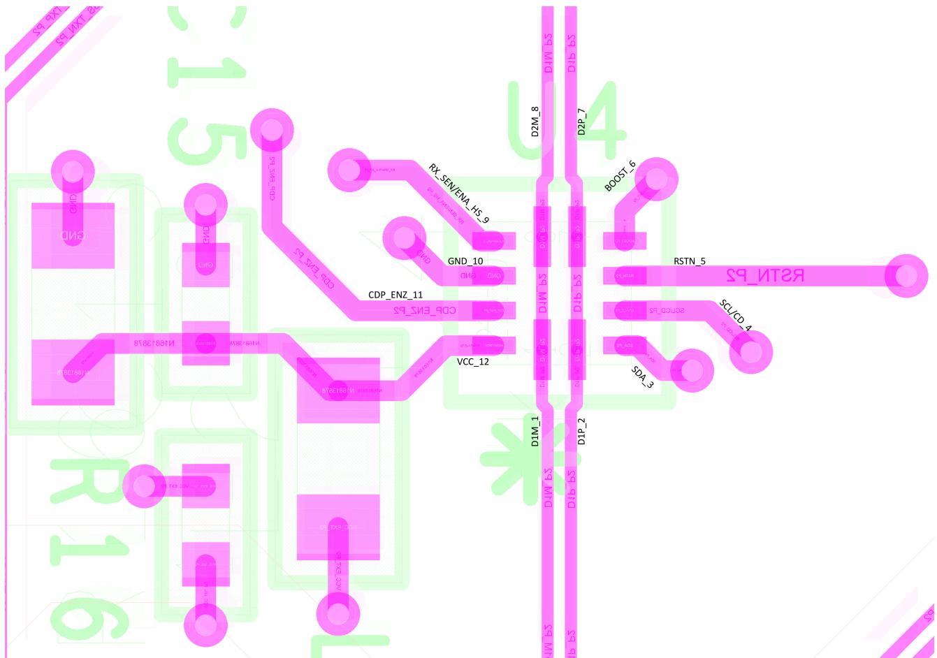
Figure 8-22. Layout Example
