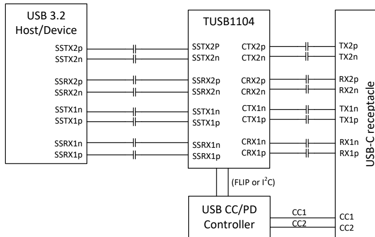
Simplified Schematic
