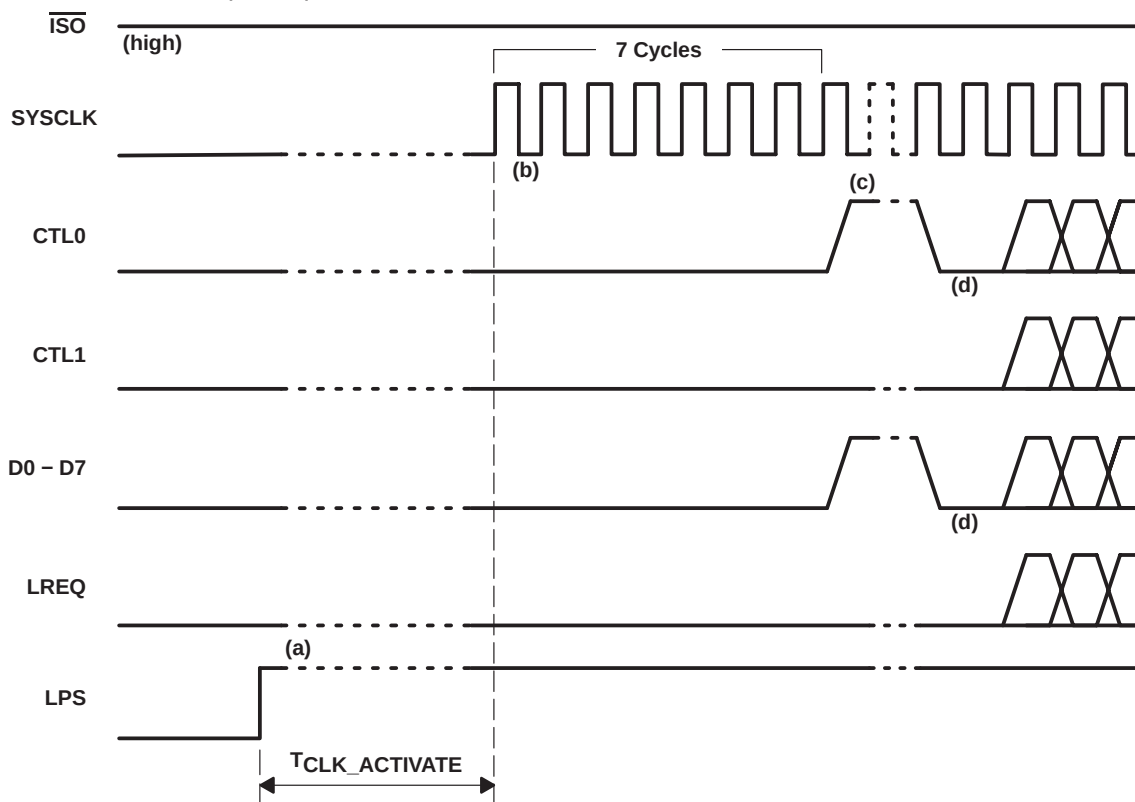
Figure 28. Interface Initialization, \overline{\text{ISO}} High
