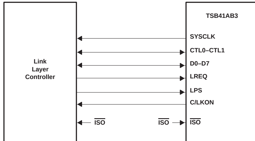
Figure 14. PHY-LLC Interface
