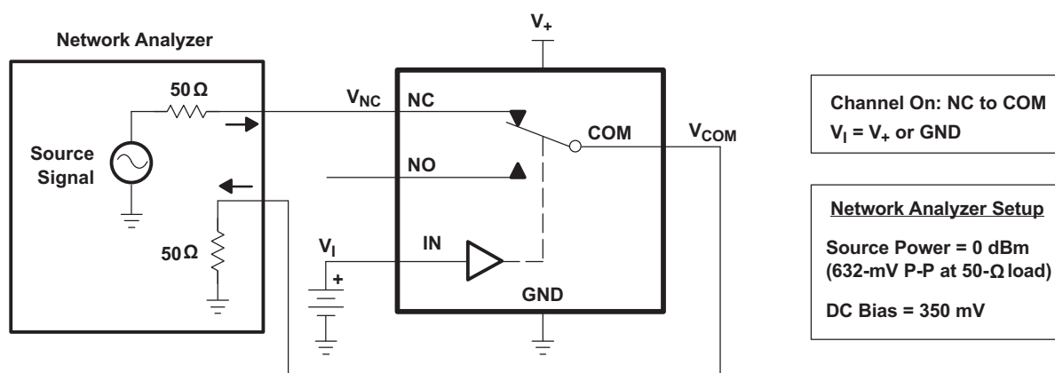
Figure 20. Bandwidth (BW)
