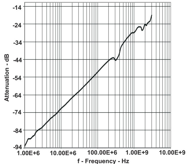
Figure 6-2. OFF Isolation vs Frequency
