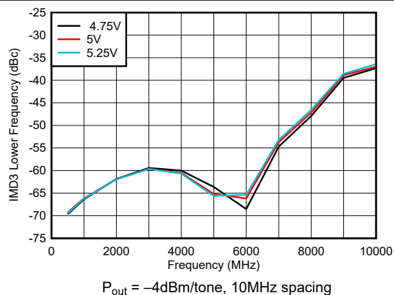
Figure 5-12. IMD3 Lower Across Supply Voltage
