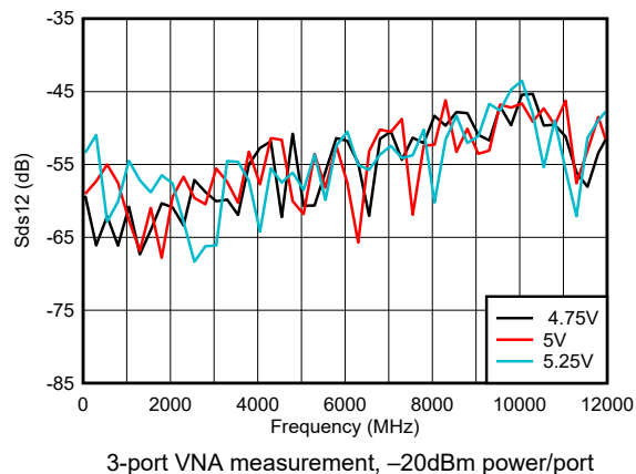
Figure 5-8. Reverse Isolation Across Supply Voltage
