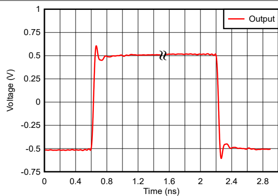
Figure 5-49. Step Response
